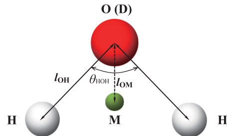
Fig. 3 Molecular structure of the SWM4-NDP water model
