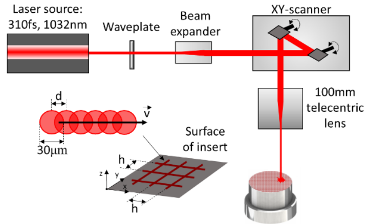
Figure 1. Beam line components and the laser scanning strategy.
