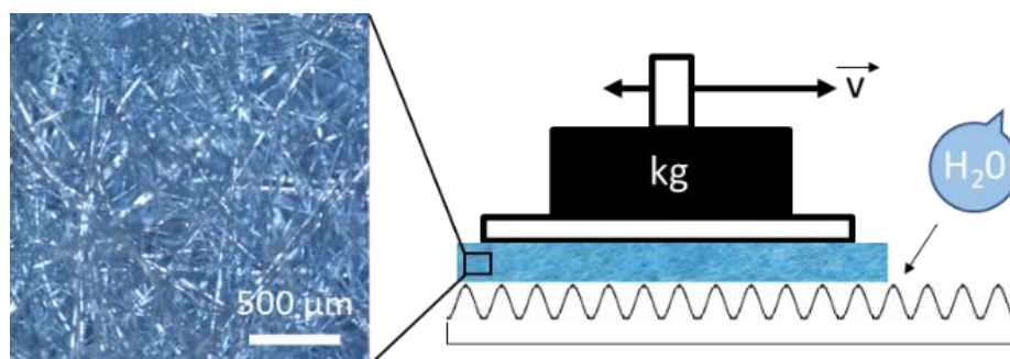
Figure 3. Washability tester with multipurpose cloth.
