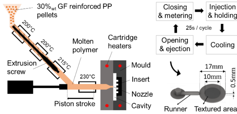
Figure 2. Micro injection moulding setup and stages together with the design of the PP replicas.
