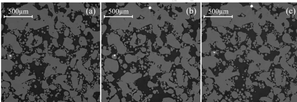
Figure 16. X \mu CT radiographs ( P=150W , v=2500mm/s , h=105\mu m , t=60\mu m ) showing no change in interconnected porosity (dark regions) with treatment: as-built (a); HIPped (b); HIPped + T6'd (c)
