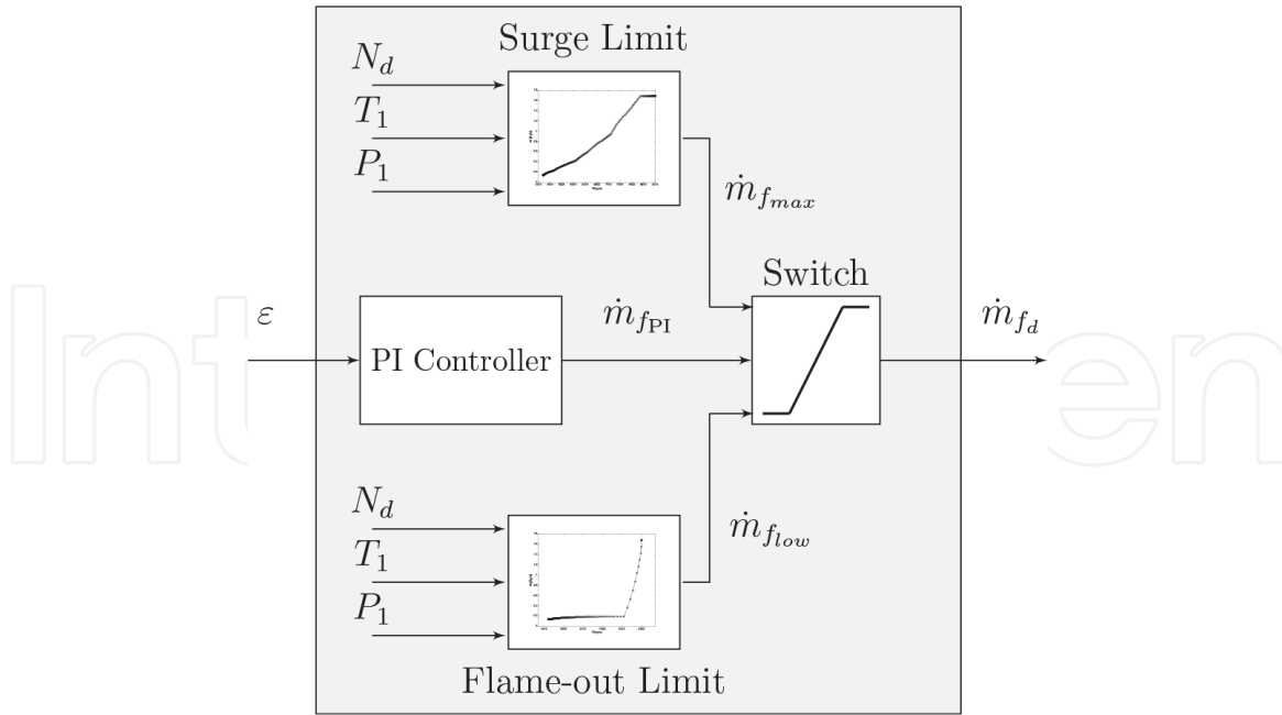
Figure 7. Detailed block diagram of the controller subsystem with the surge and flame-out limiting functions implemented as look-up tables [14].
