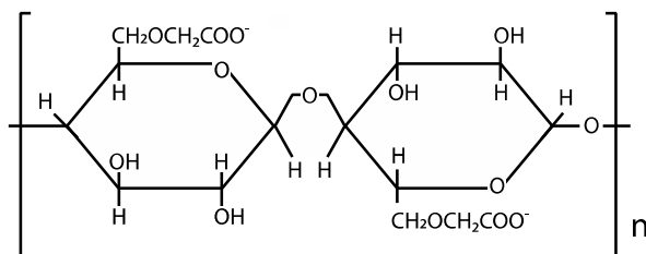
Figure 2: Carboxymethylcellulose structure
