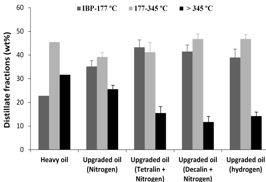
Figure 3. Feed oil and upgraded oils distillate fractions.
