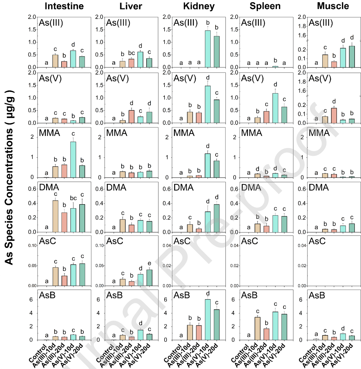
Figure 2. As species concentrations in intestine, liver, kidney, spleen, and muscle tissues of crucian carp after 100 \mu\text{g g}^{-1} As(III) and As(V) dietborne exposure for 10 d and 20 d. Values are means \pm SD ( n = 7 ). Different letters indicate significant differences among treatments ( p < 0.05 ).
