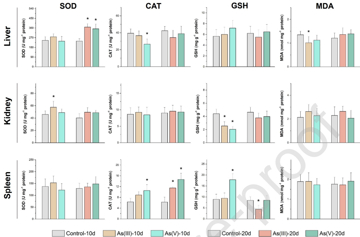
Figure 3. SOD, CAT activities and GSH, MDA contents in liver, kidney, and spleen of crucian carp after 50 µg g -1 As(III) and As(V) dietborne exposure for 10 d and 20 d. Values are means ± SD (n = 7). Significant differences versus control are marked with * ( p < 0.05 ).
