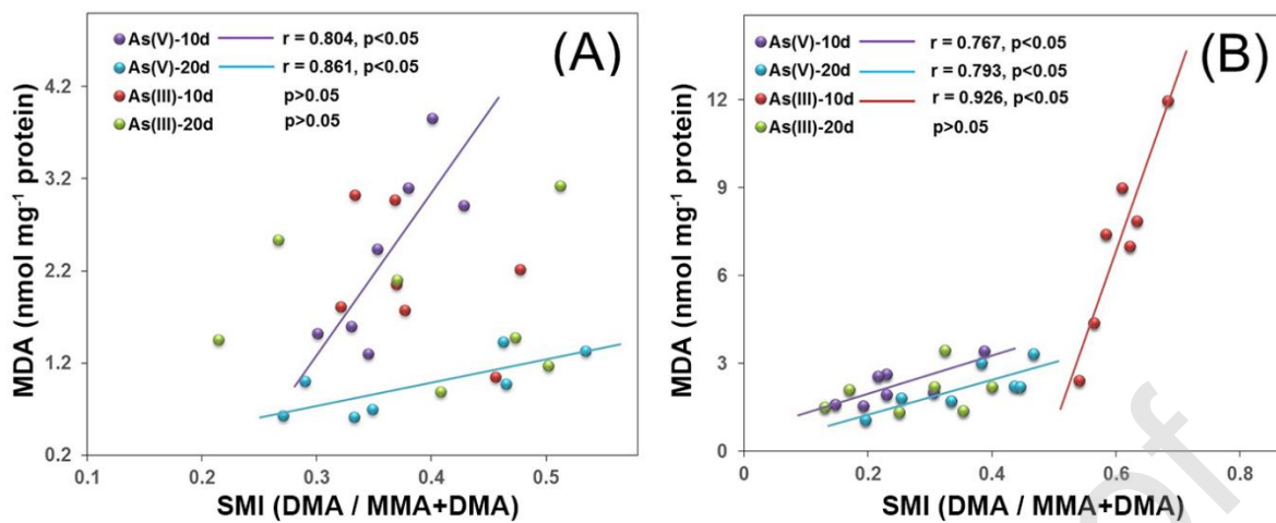
Figure 5. Correlation between secondary methylation index (SMI), which was calculated as \text{DMA}/(\text{MMA} + \text{DMA}) , and malondialdehyde (MDA) in liver (A) and kidney (B) of crucian carp after 100 \mu\text{g g}^{-1} As(III) and As(V) dietborne exposure for 10 d and 20 d.
