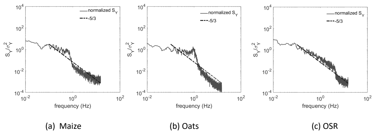
Figure 7 Typical streamwise displacement spectra
