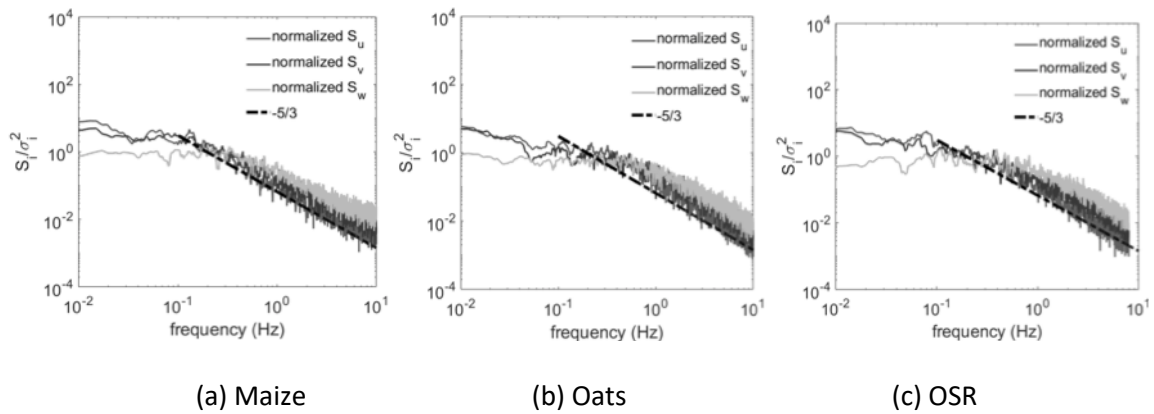
Figure 6 Wind velocity component power spectra at crop height.
