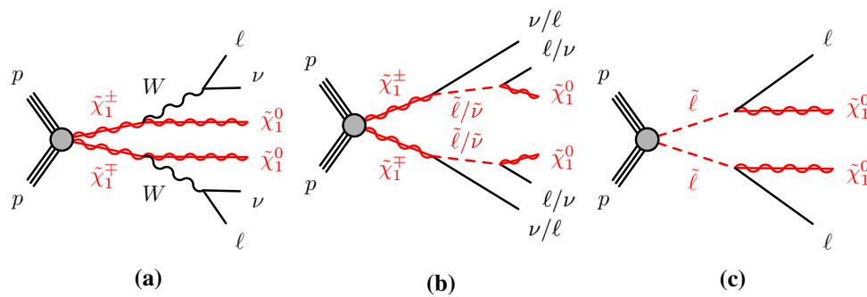
Fig. 1 Diagrams of the supersymmetric models considered, with two leptons and weakly interacting particles in the final state: a \tilde{\chi}_1^+ \tilde{\chi}_1^- production with W -boson-mediated decays, b \tilde{\chi}_1^+ \tilde{\chi}_1^- production with slepton/sneutrino-mediated decays and c slepton pair production. In the model with intermediate sleptons, all three flavours
