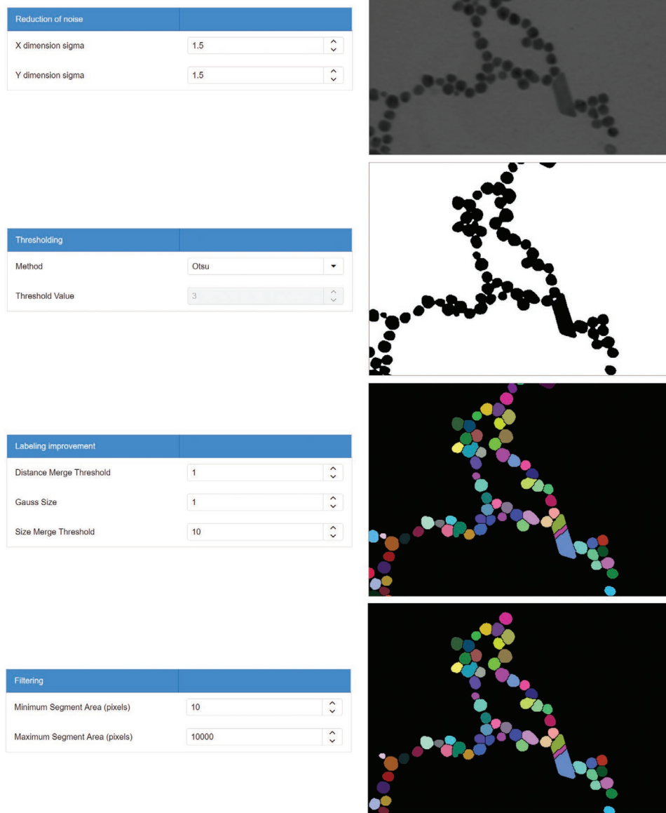
Figure 4. Screenshot of the four steps for parameter tuning (reduction of noise, thresholding, labeling improvement, filtering) with the default values shown. Users can tune these values, as per their needs and expertise level.
