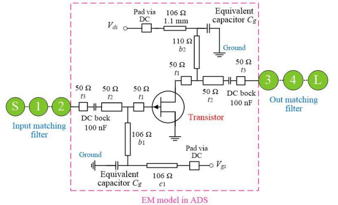
Fig. 5 On-chip transistor circuit schematic of the filter-amplifier.
