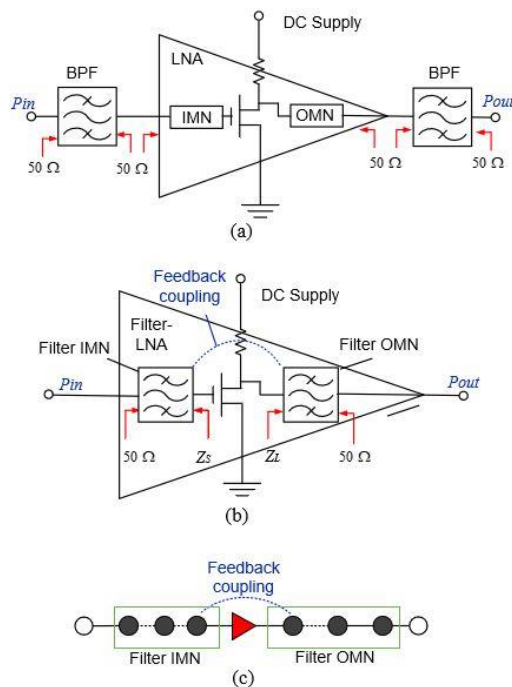
Fig. 1. (a) Conventional cascaded filters and amplifier with 50\ \Omega interfaces between them; (b) The proposed integrated filter-amplifier, with feedback coupling between the drain and gate; (c) The coupling topology representation of (b).
