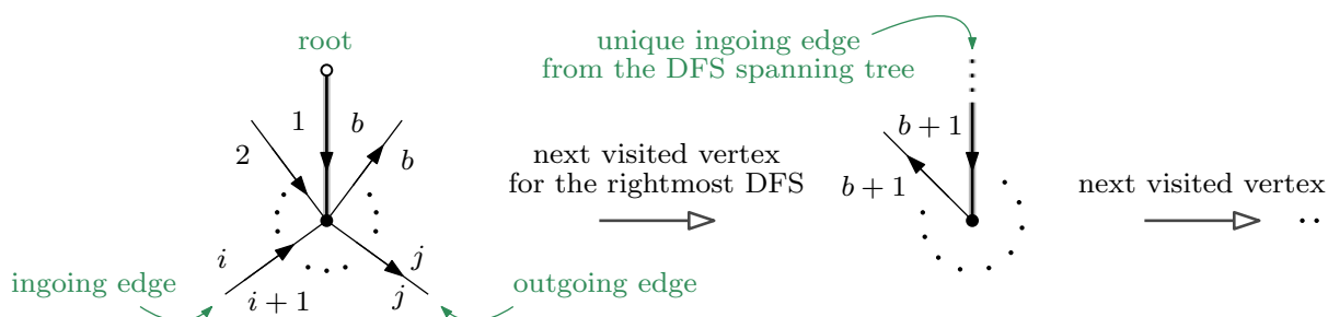
Figure 24: DFS-labeling procedure
