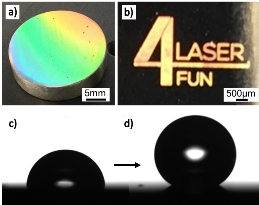
Figure 8. The uniform structural colours of triangular LIPSS over large area (a) and micro-scale logo writing (b). The contact angle of 6 \mu\text{l} water drops on untextured (c) compared to textured (d) X6Cr17.
