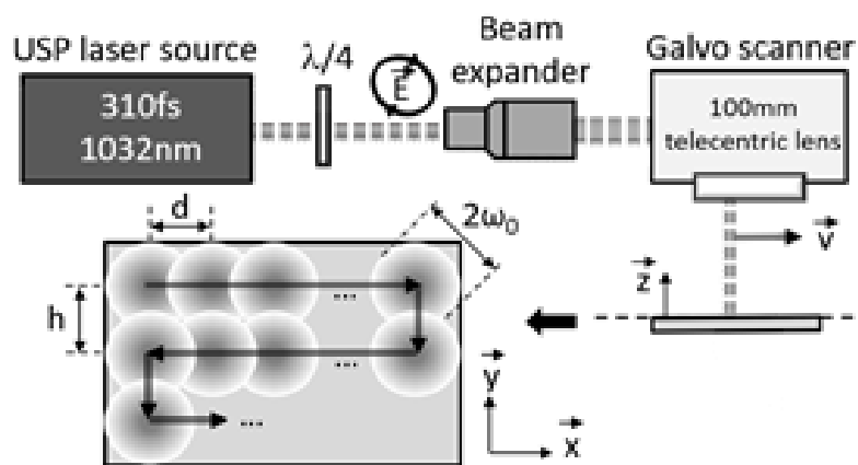
Figure 2. Beam line components and raster scan strategy.
