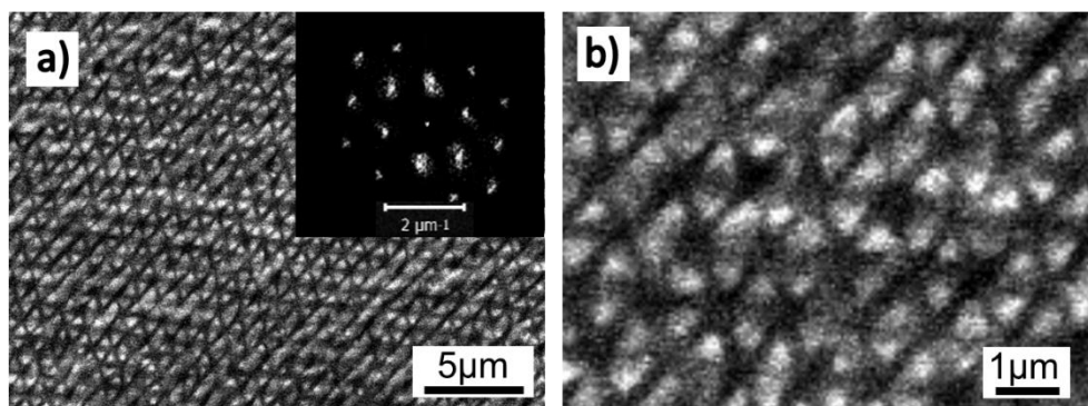
Figure 6. SEM pictures with corresponding FFT (a) and detailed view (b) of triangular LIPSS on Ti-6Al-4V ( h = 2 \mu\text{m} , \varphi_0 = 54 \text{ mJ/cm}^2 , N = 442 , \varphi = 23.9 \text{ J/cm}^2 ).
