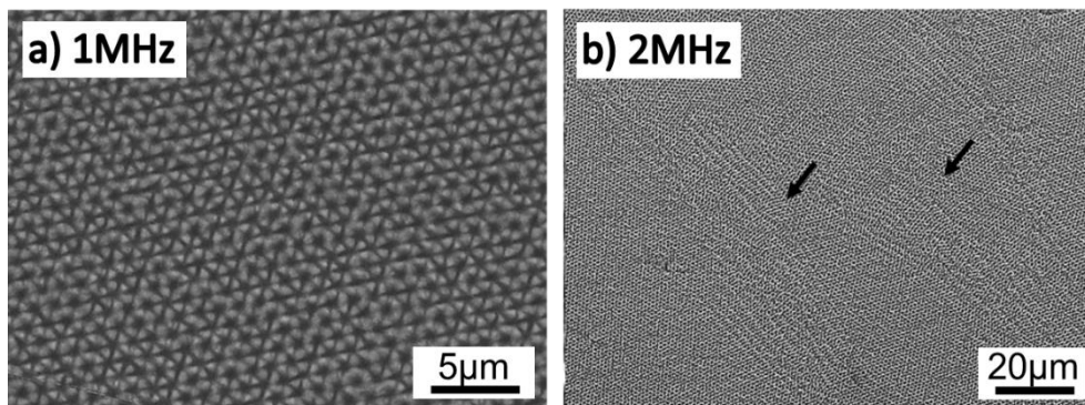
Figure 7. MHz processing of triangular LSFL on X6Cr17 at fixed h = 2 \mu\text{m} , \varphi_0 = 100 \text{ mJ/cm}^2 , for 118 pulses at 1 MHz (a) and 141 pulses at 2 MHz (b).
