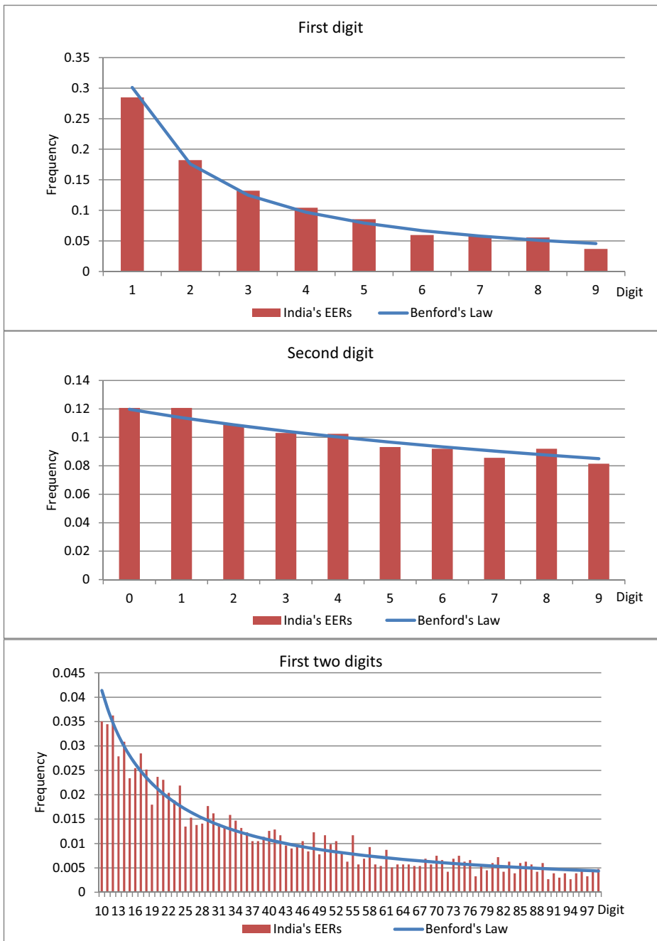
Fig. 2 Digital frequency analysis of emission reduction claims for projects in India. Plotted are the frequencies of each digit for d1 , d2 and d1d2 for EERs of CDM projects hosted in India as well as the corresponding expected frequencies from Benford's Law
