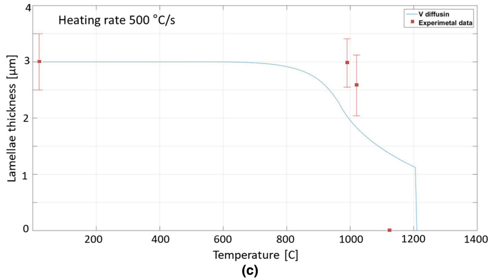
Fig. 10—Comparison of lamellar thickness predicted by numerical model (Vanadium as diffusing element) and the experimental measurements, at heating rates of (a) 5 °C/s, (b) 50 °C/s, (c) 500 °C/s.
