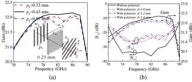
Fig. 3 Analysis of the 45° linear polarizer. (a) Simulated peak gain with different periods p_e ; (b) Simulated peak gain and |S_{11}| with and without the polarizer.
