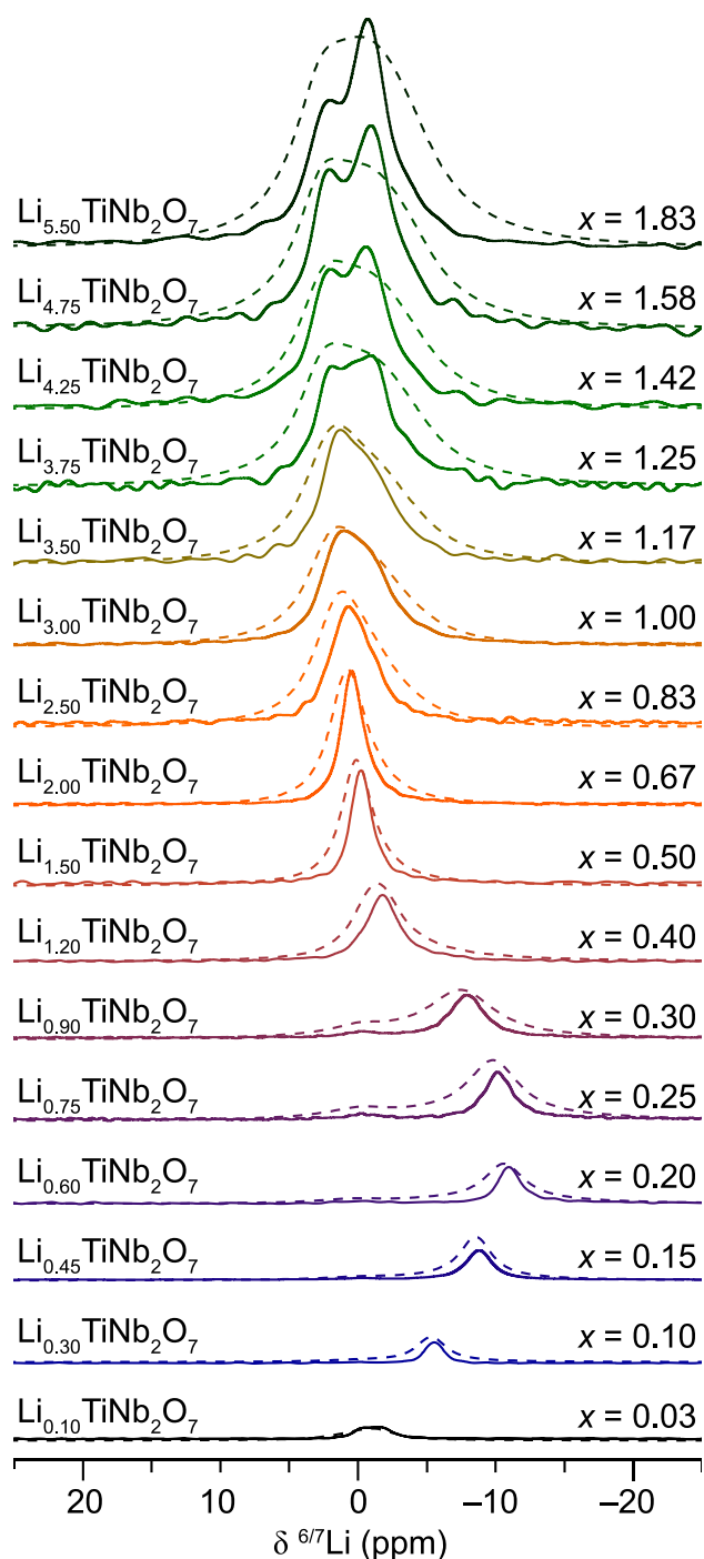
Figure 5. ^6\text{Li} (solid lines) and ^7\text{Li} (dashed lines) MAS NMR spectra of \text{Li}_x\text{TiNb}_2\text{O}_7 . Single-pulse spectra were collected in the range x = 0.10 – 5.50 ( 8 – 426 mA h \text{g}^{-1} ) at an MAS frequency of 12.5 kHz and B_0 = 11.7 T.
