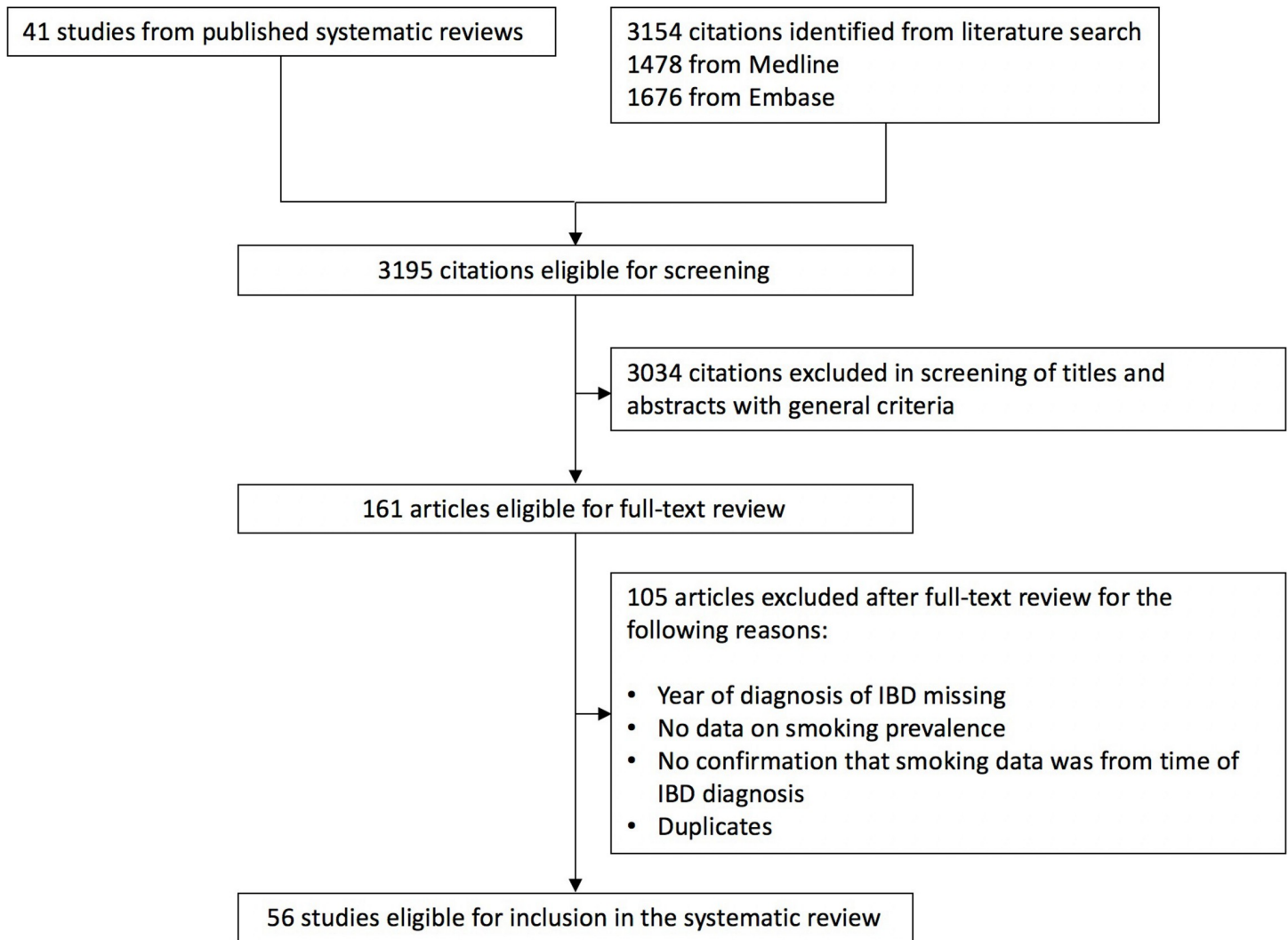
Fig 1. Study selection.
