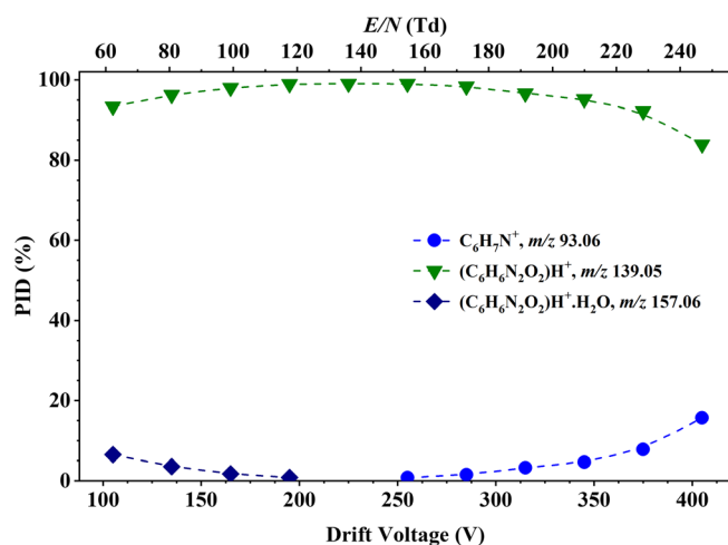
Figure 6. Percentage product ion distribution resulting from the reaction of 4-nitroaniline with \text{H}_3\text{O}^+(\text{H}_2\text{O})_n ( n=0, 1 and 2) as a function of the reduced electric field from 60 to 250 Td
