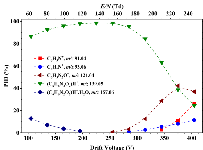
Figure 3. Percentage product ion distribution (PID in %) resulting from the reaction of 2-nitroaniline with \text{H}_3\text{O}^+(\text{H}_2\text{O})_n ( n=0 and 1) as a function of the reduced electric field from 60 to 250 Td
