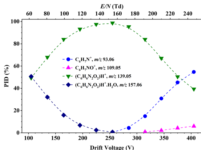
Figure 5. Percentage product ion distribution resulting from the reaction of 3-nitroaniline with \text{H}_3\text{O}^+(\text{H}_2\text{O})_n ( n=0 and 1) as a function of the reduced electric field from 60 to 250 Td
