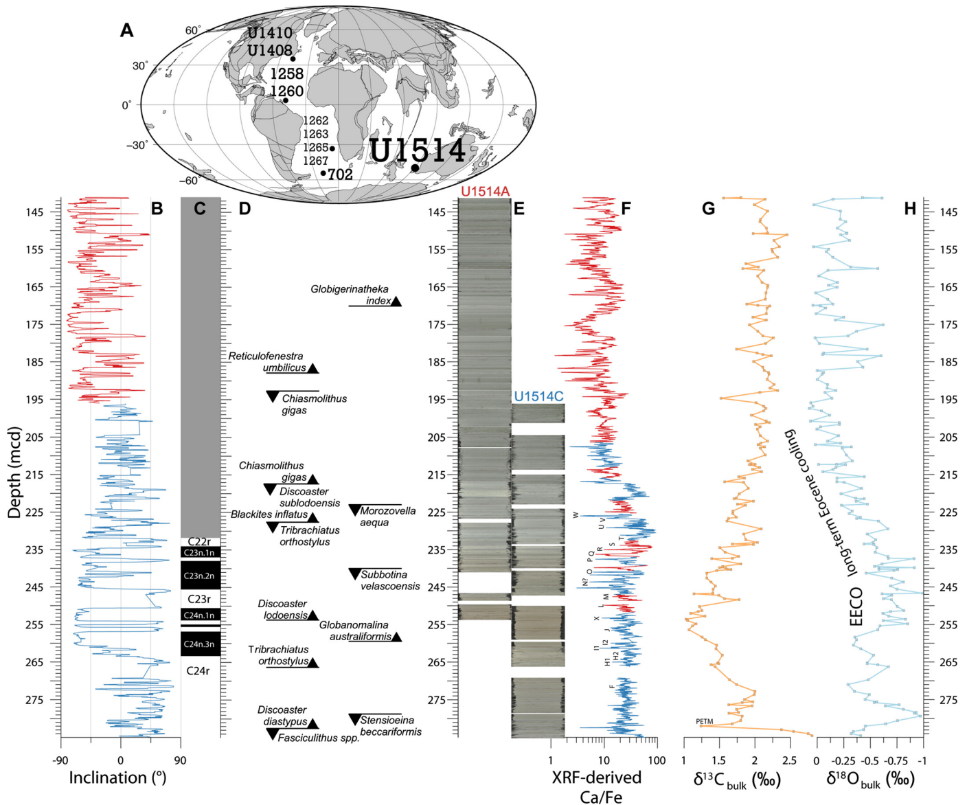
Fig. 1. (A) Location of Site U1514 and other deep-sea sites used for timescale reconstruction in the early and middle Eocene (paleomap \sim 45 Ma, www.ods.de ). (B) Downhole NRM20mT inclinations (after 20 mT demagnetization) from Holes U1514A (red) and U1514C (blue). (C) Magnetostratigraphic interpretation (white = reversed, black = normal, gray = undetermined). (D) Shipboard biostratigraphic events (Huber et al., 2019). (E) Core images stitched together with IODP CoreImage (Drury et al., 2018). (F) XRF-derived Ca/Fe ratio according to the shipboard splice between Holes U1514A (red) and U1514C (blue). Early Eocene hyperthermals follow the naming scheme of Cramer et al. (2003). (G-H) Bulk sediment carbon isotope and oxygen isotope data. (For interpretation of the colors in the figure(s), the reader is referred to the web version of this article.)
