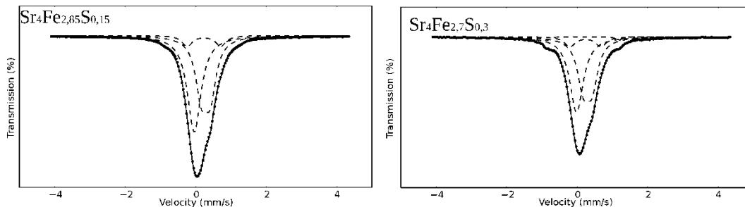
Figure 8. ^{57}\text{Fe} Mössbauer spectrum from \text{Sr}_4\text{Fe}_{2.85}\text{S}_{0.15}\text{O}_{10-\delta} and \text{Sr}_4\text{Fe}_{2.7}\text{S}_{0.3}\text{O}_{10-\delta} at 298 K
