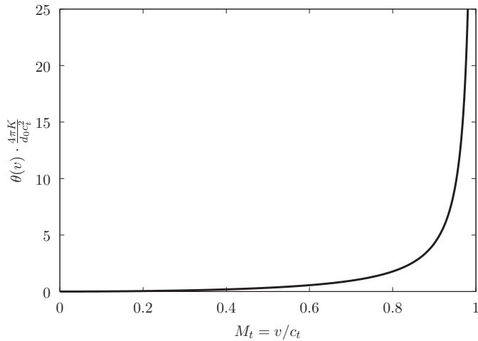
Fig. 2. Evolution of the temperature field of a moving dislocation in the immediacy of the core of the dislocation.
