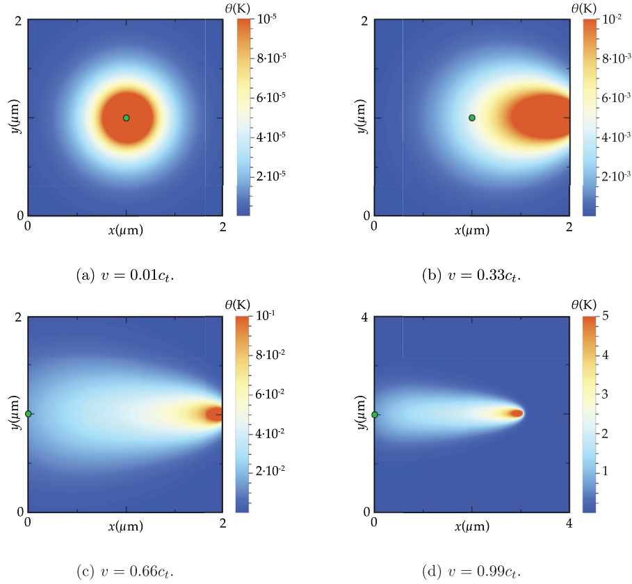
Fig. 1. Temperature fields for a uniformly moving dislocation, relative to a base temperature T_0 = 298 K. The parameters of pure aluminium have been used, with K = 205 W/m K, c_t = 2980 m/s, \kappa_t = 9.7 \times 10^{-5} m 2 /s, d_0 = 2 \times 10^{-5} Pas. The initial position of the dislocation is marked with a green circle, and it moves in the x direction at the specified uniform speed. The plots display the resulting temperature field at instant t = 1 ns. (For interpretation of the references to colour in this figure legend, the reader is referred to the web version of this article.)
