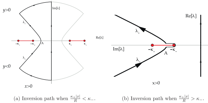
Fig. 4. Inversion paths.
