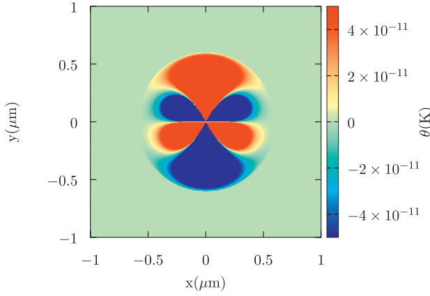
Fig. 5. Uncoupled temperature field for an injected edge dislocation. The dislocation was injected at the origin, and the instant in time represented is 0.1 ns; the material constants of FCC Al have been used.
