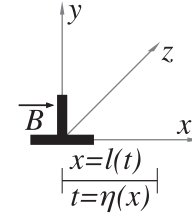
Fig. 3. Thermoelastic system. The dislocation of Burgers vector B is injected at the origin, and glides along the x axis following a certain x = l(t) history. The system's material properties are its two elastic Lamé constants \Lambda and \mu , its density \rho , its linear expansion coefficient \alpha and its thermal conductivity K .
