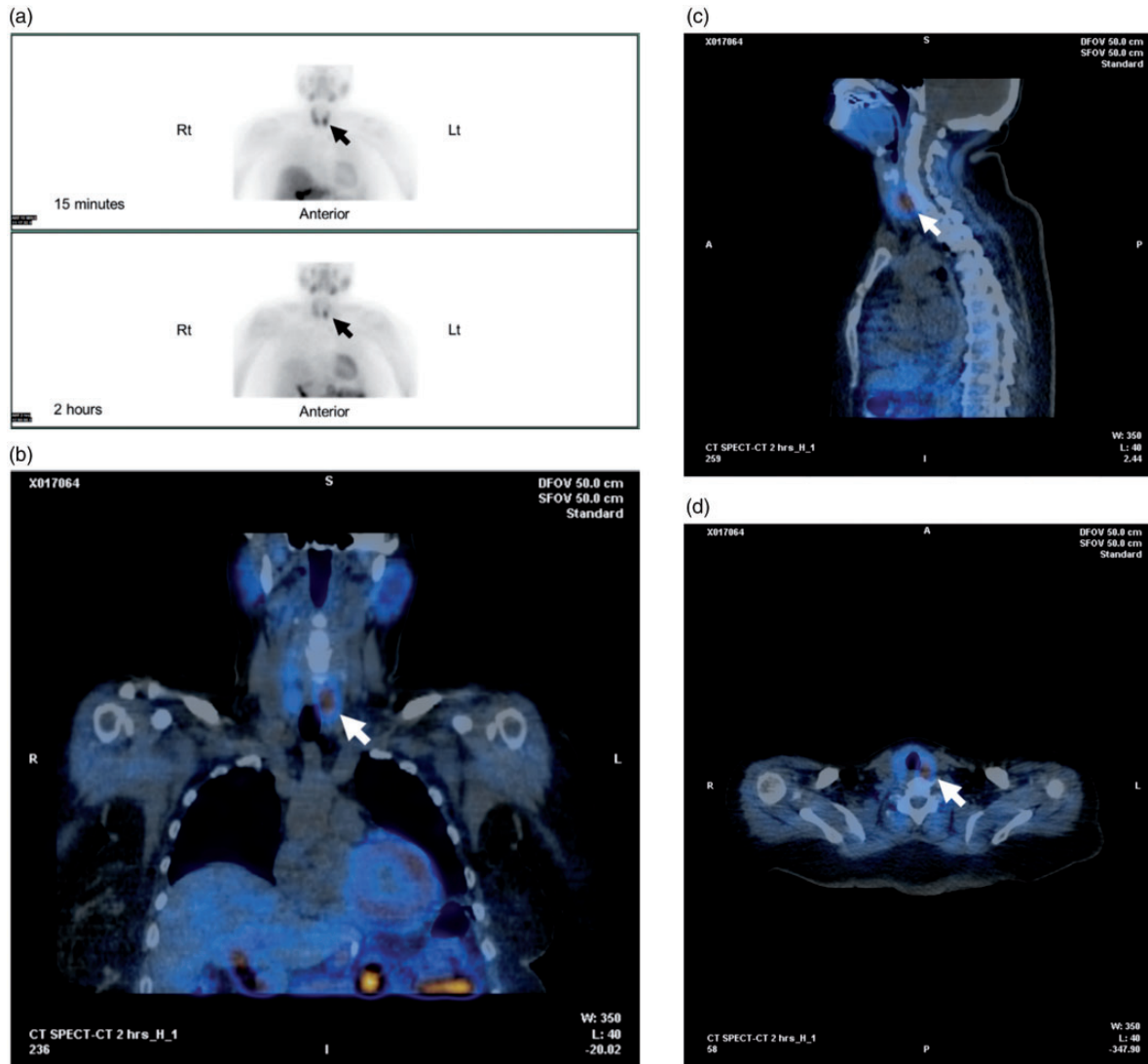
Figure 2. Anterior maximum intensity projection images from early (15 min) and delayed (2 h) phases of SPECT in the same woman undergoing ultrasound scan (Figure 1) showing delayed washout of radiotracer in the left inferior parathyroid adenoma (a). Delayed-phase coronal (b), sagittal (c) and axial (d) fused 99m Tc-sestamibi-SPECT/CT images confirm this parathyroid adenoma localising posterior to the inferior pole of the left lobe of thyroid (c,d).
