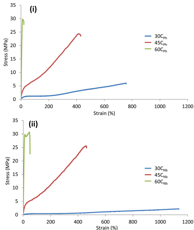
Fig. 2 Exemplar stress–strain curves of (i) C_{Ph} -based TPEUs and (ii) C_{Nb} -based TPEUs. Experiments were conducted at ambient temperature ( \sim 25\text{ }^{\circ}\text{C} ) at an elongation rate of 5\text{ mm min}^{-1} until failure.
