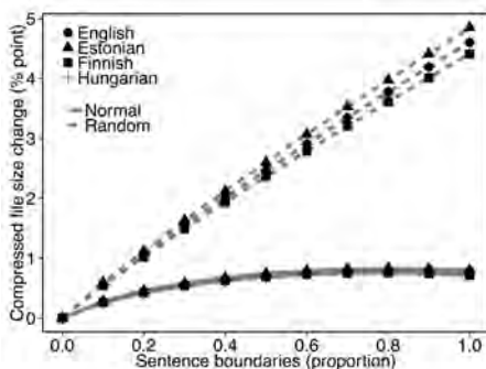
Figure 1. Relation between sentence boundaries and file size change.
