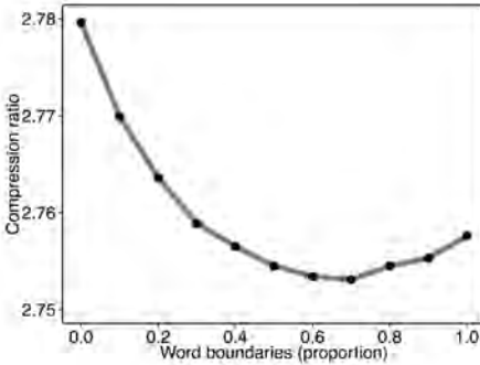
Figure 11. Compression ratios for boundaries added at low frequency contexts.
