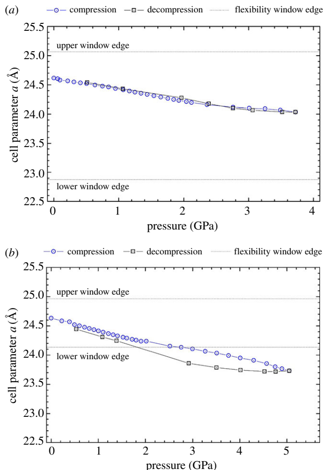
Figure 2. Cell parameter a as a function of pressure for (a) the empty and (b) the filled zeolite Na-X. Blue circle data points correspond to the compression cycle, and black squares to the decompression. Also shown are the edges of the flexibility window as simulated in the GASP software.
