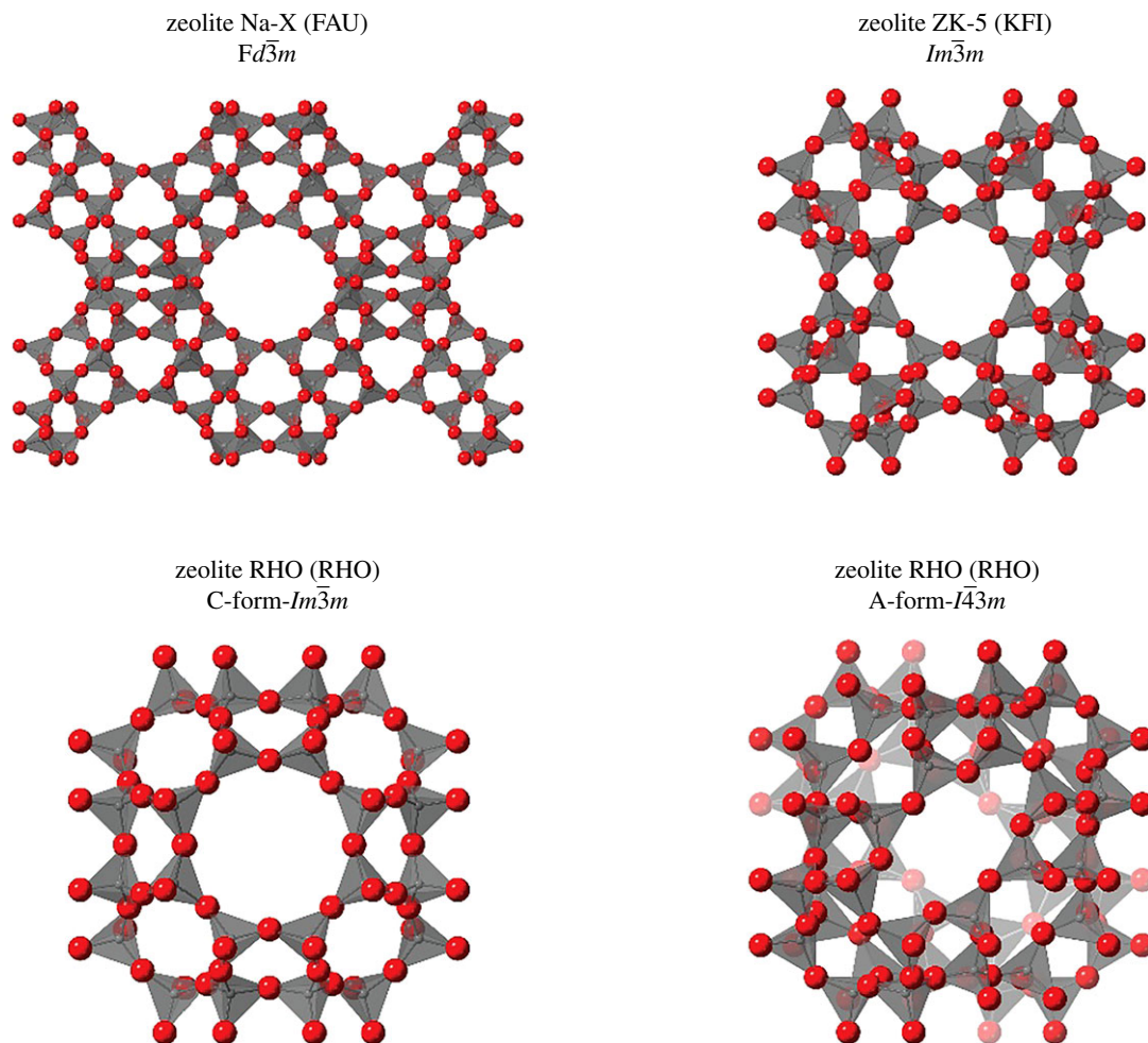
Figure 1. The structures and space groups of zeolites Na-X, ZK-5 and the C- and A-forms of zeolite RHO. The framework topology is indicated in parentheses. Oxygen atoms are shown as red spheres, and SiO_4 tetrahedra as translucent solids.
