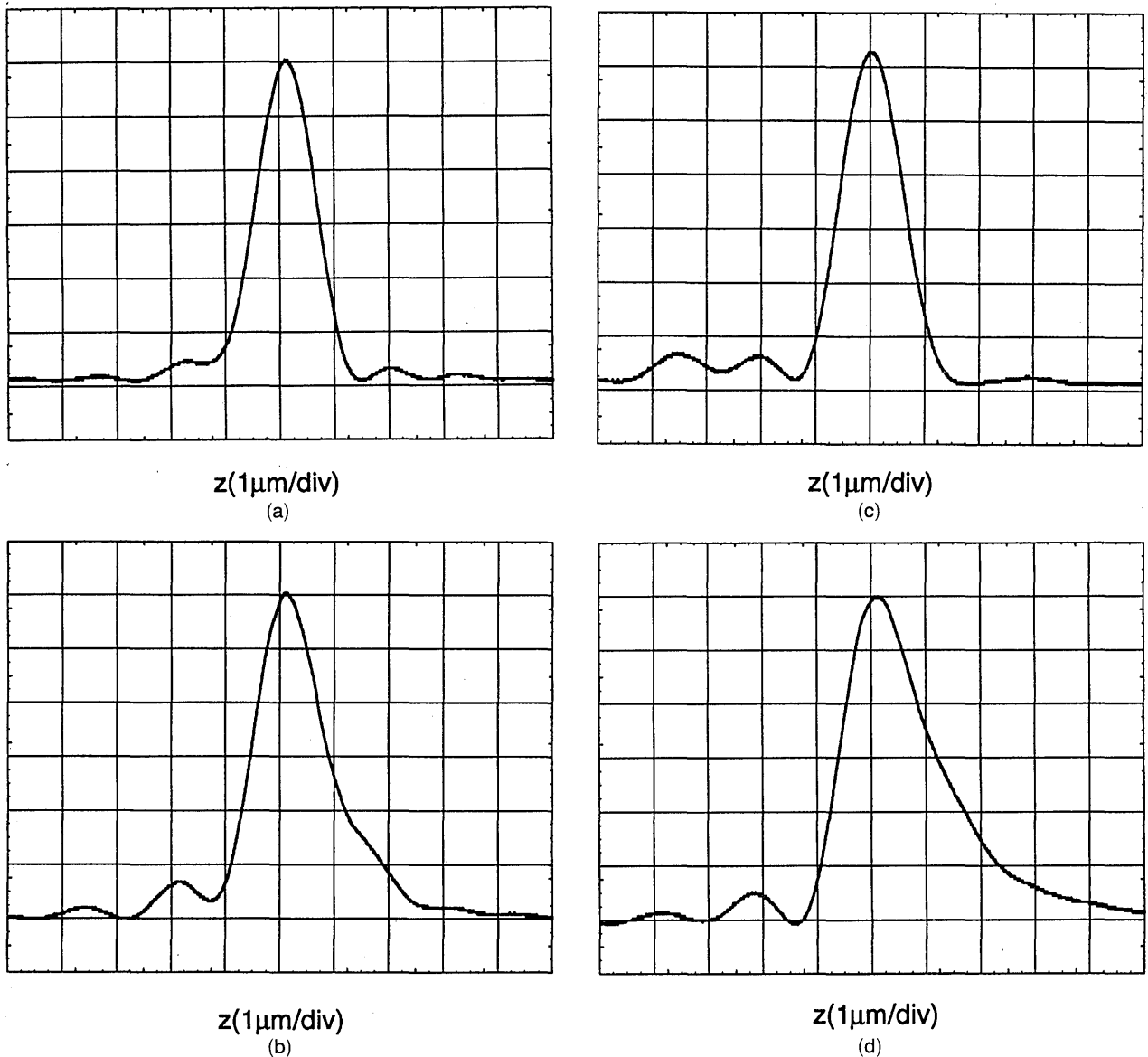
Fig. 12. Measured axial responses for different diameters ( D ) of the entrance pupil of the objective: (a) D = 6.5 mm with a number 1\frac{1}{2} cover glass of thickness 0.17 mm, (b) D = 6.5 mm with a number 1 cover glass of thickness 0.12 mm, (c) D = 5 mm with a number 1 cover glass of thickness 0.12 mm, (d) D = 4.5 mm with a number 1 cover glass of thickness 0.12 mm.
