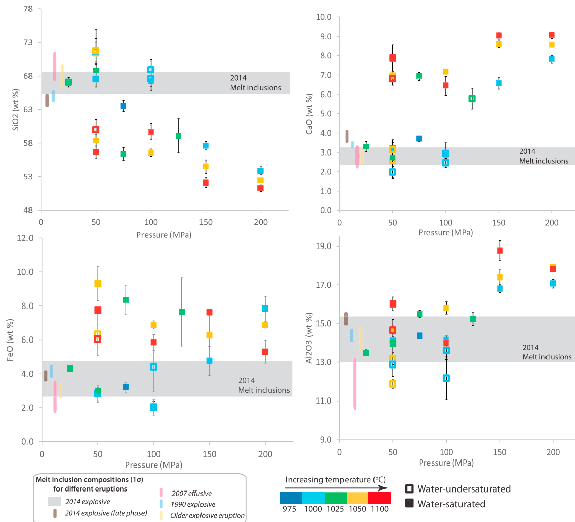
Figure 4. Dashed line/open symbol: where \text{XH}_2\text{O} is <1 . Grey band = 1 standard deviation of melt inclusion composition. Error bar indicate 1 standard deviation of the glass data.
