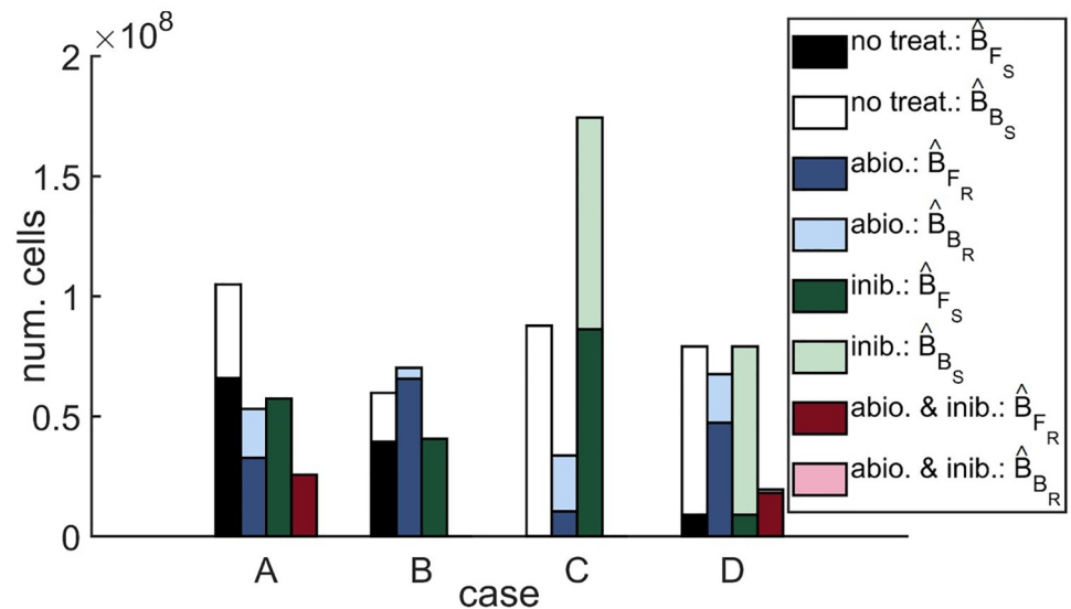
Fig 2. Steady-state solutions. Four stacked bars are plotted for each case: the first bar shows the number of free and bound susceptible bacteria, \hat{B}_{FS} = VB_{FS} and \hat{B}_{BS} = A_r B_{BS} , at steady-state in the untreated scenario; the second bar shows the number of free and bound resistant bacteria, \hat{B}_{FR} = VB_{FR} and \hat{B}_{BR} = A_r B_{BR} , at steady-state in the antibiotic only scenario; the third bar shows the number of free and bound susceptible bacteria at steady-state in the inhibitor only scenario, and the fourth bar shows the number of free and bound resistant bacteria at steady-state in the antibiotic and inhibitor scenario. There are no resistant bacteria at steady-state in the absence of antibiotic, nor are there any susceptible bacteria at steady-state in the presence of antibiotic. Thus, the combined height of the bars in each stack gives the total number of bacteria, B_T . Treatment with antibiotics alone reduces the total bacterial burden in Cases A, C and D, and increases it in Case B. Treatment with inhibitors alone reduces the total bacterial burden in Cases A and B, increases it in Case C and has a negligible effect in Case D. Treatment with both antibiotics and inhibitors eliminates the bacterial burden in Cases B and C, and reduces it more than either treatment in isolation in Cases A and D. Steady-state solutions to Eqs 1–10 were calculated using Maple, neglecting the Heaviside step functions which prevent the logistic growth of bacteria when their population size goes beneath one. Parameter values: \tilde{\psi}_{Bac} = 0 \text{ hr}^{-1} , \tilde{\psi}_I = 0 \text{ hr}^{-1} , \lambda = 0 \text{ cm}^3 \text{ cell}^{-1} \text{ hr}^{-1} , \rho = 0 \text{ hr}^{-1} , \omega = 1 , A = 0 or 8 \mu\text{g cm}^{-3} , and I_{Fmit} = 0 or 6.12 \times 10^7 \text{ inhib. cm}^{-3} . See Tables 2–4 for the remaining parameter values.
