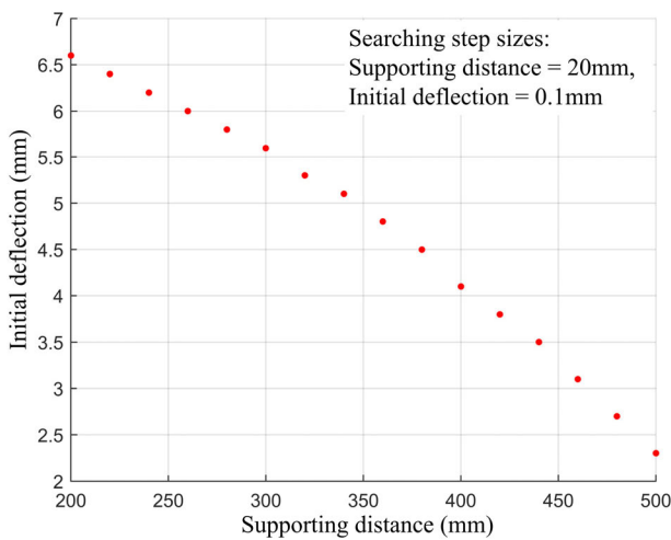
FIGURE 3. Deflection-distance distribution avoiding the unexpected deformation.
