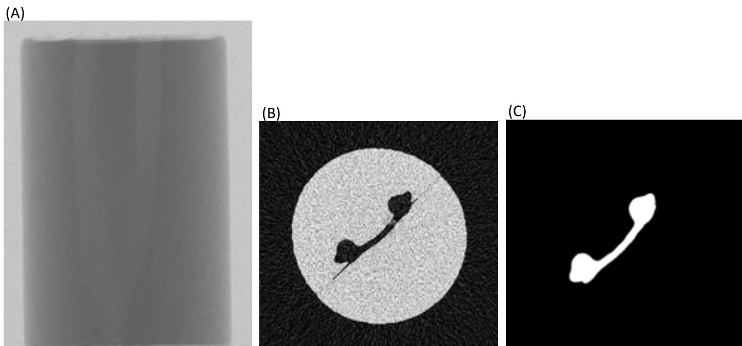
Figure 1a: (A) Micro-CT scanning of non-obturator 3D printed plastic block, (B) NRecon reconstructed slice of non-obturator 3D printed plastic block, (C) Extraction of canal volume of 3D printed plastic block using Image J software. Canals connected by complete isthmus seen.
