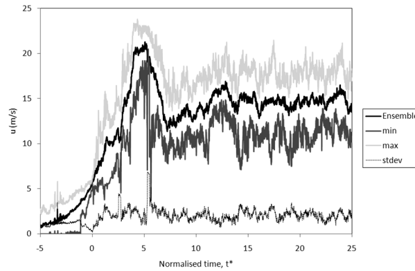
Fig. 10 Ten test ensemble average, X/D = 1.25 , Y/D = 0.021 , H/D = 2 using ‘flaps control’ method
