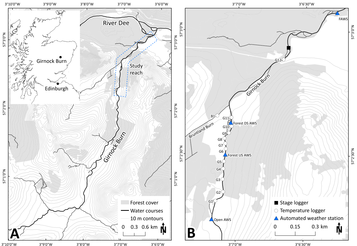
Fig. 1. a) Girnock Burn with location of study reach marked (blue dashed polygon). b) Location of temperature loggers, automated weather stations and Marine Scotland gauging station within study reach.
