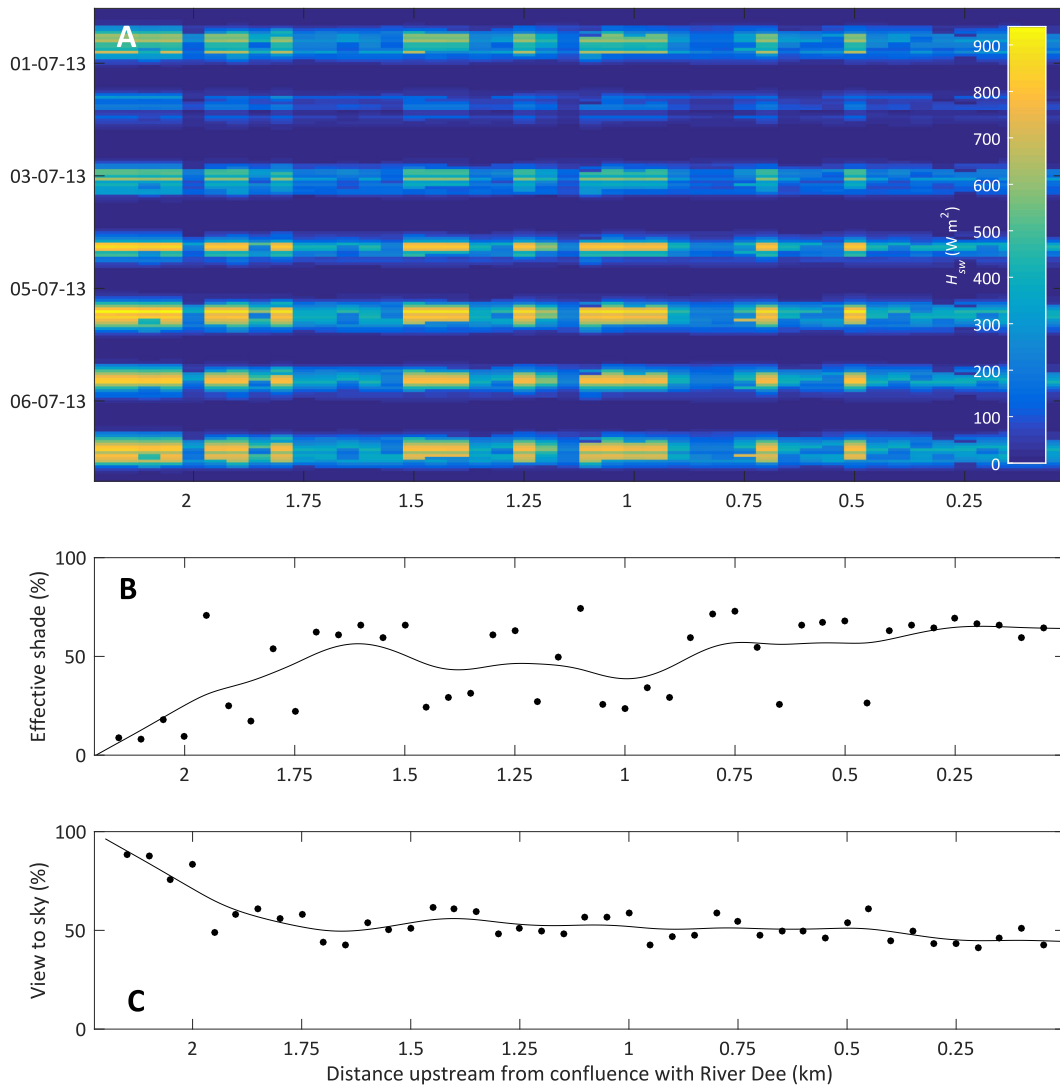
Fig. 4. Variability in a) computed H_{sw} , received at the stream surface following application of Heat Source shading routines to SfM-derived tree heights, b) time-averaged effective shade and c) view to sky (VTS). Solid lines in b) and c) indicate LOESS-smoothed average effective shade and VTS.
