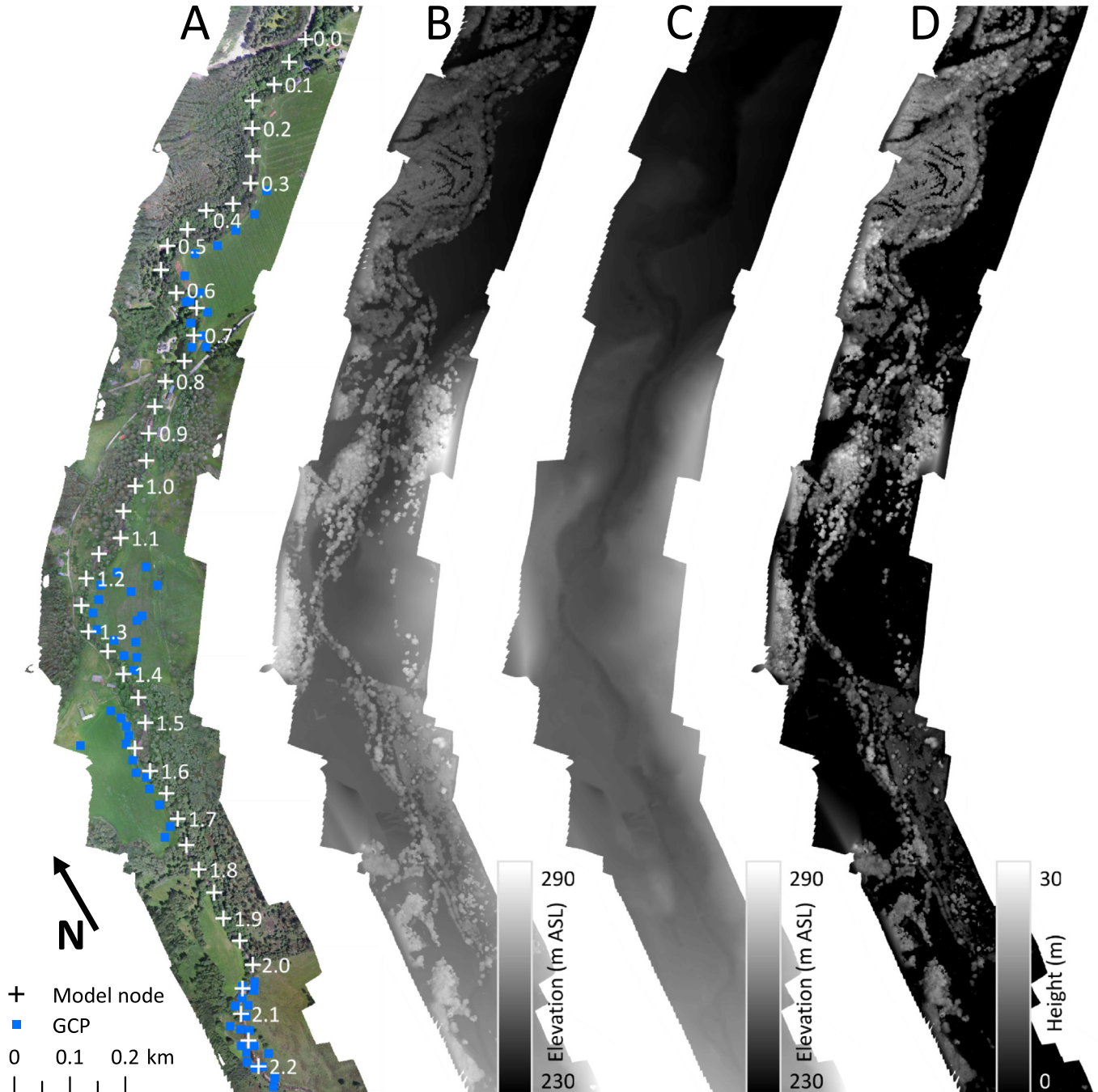
Fig. 2. a) sUAS orthophoto of study reach with model nodes and ground control points (GCPs) marked. b) SfM-derived digital surface model (DSM) of study reach. c) Digital terrain model (DTM) created through from classification of SfM ground points. d) Tree height raster generated by subtracting DTM from DSM. Note north offset of -30^\circ .
