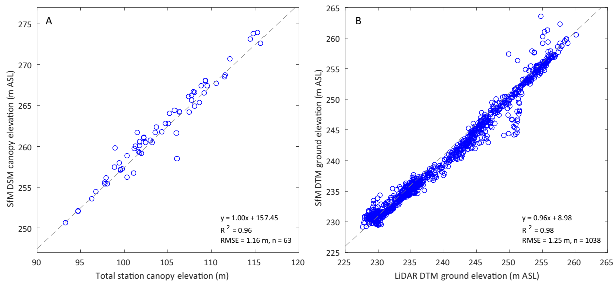
Fig. 3. a) Comparison between SfM-derived tree canopy elevations (extracted from DSM) and total station observations (field measurements). b) Comparison between SfM and LiDAR-derived below-canopy elevations (extracted from DTM). Total station elevations are given relative to the total station (set at 100 m in the X,Y and Z coordinates), all other elevations are relative to mean sea level.
