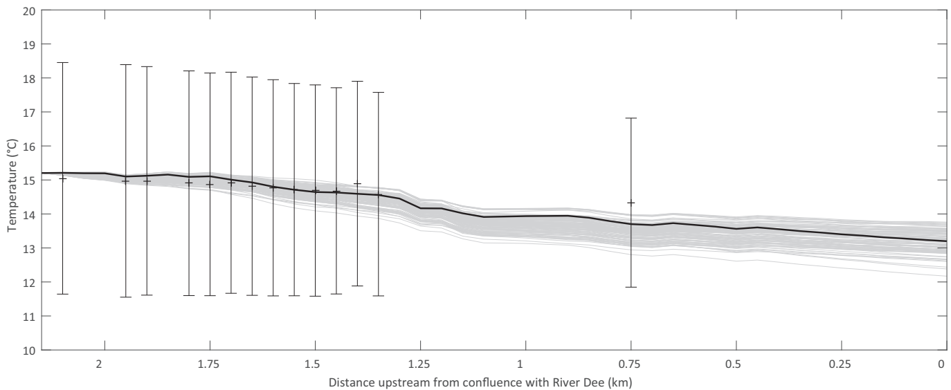
Fig. 5. Time-averaged river temperature long profile for 100 best optimisation runs (based on RMSE). Best model (lowest mean RMSE) given by thick black line. Vertical bars give standard deviation of temperatures observed at logger sites; crosses give mean recorded river temperature.
