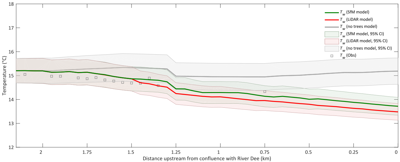
Fig. 7. Time-averaged temperature long profiles for Girnock Burn simulated with SfM model (green line), LiDAR model (red line) and no trees model (grey line). Shaded area represents 95th percentiles around mean. Note that simulations for the SfM and LiDAR models upstream of 1.7 km are identical.
