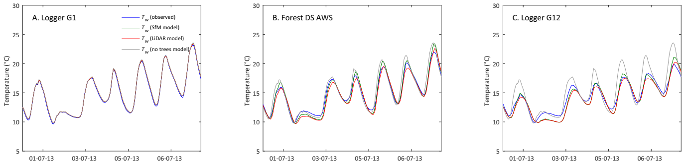
Fig. 6. Observed vs. simulated (SfM, LiDAR and no trees models) stream temperature at a) upstream, b) mid-stream and c) downstream logger sites. Note that simulations for SfM and LiDAR models at logger G1 are identical.
