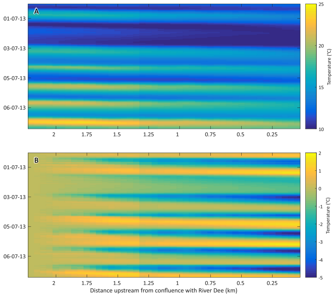
Fig. 8. Spatio-temporal variability in simulated water temperature for SfM model showing a) absolute temperature and b) instantaneous difference between 1st and nth model nodes.
