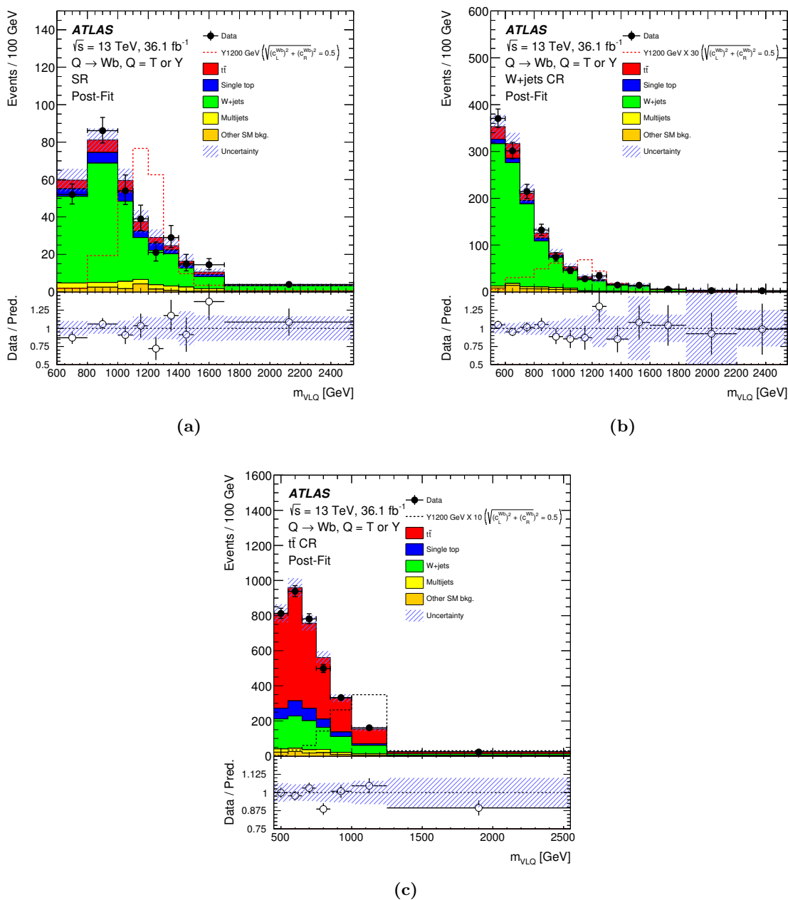
Figure 6. Distribution of the VLQ candidate mass, m_{\text{VLQ}} , in (a) the SR, (b) the W +jets CR, and (c) the t\bar{t} CR, after the fit to the background-only hypothesis. The first and last bin include the underflow and overflow respectively. The lower panels show the ratios of data to the fitted background yields. The error bars represent the statistical uncertainty in the data. The band represents the total systematic uncertainty after the maximum-likelihood fit. An example distribution for a Y signal with a coupling of \sqrt{(c_L^{Wb})^2 + (c_R^{Wb})^2} \approx 0.5 without considering any interference effects is overlaid; for better visibility, it is multiplied by a factor of 30 in the W +jets CR and by a factor of 10 in the t\bar{t} CR. While the total uncertainty decreases when performing the fit, the total uncertainty in the bins around 1450-1600 GeV and 1850-2200 GeV in (b) does not decrease due to significant statistical MC uncertainties in these two bins.
