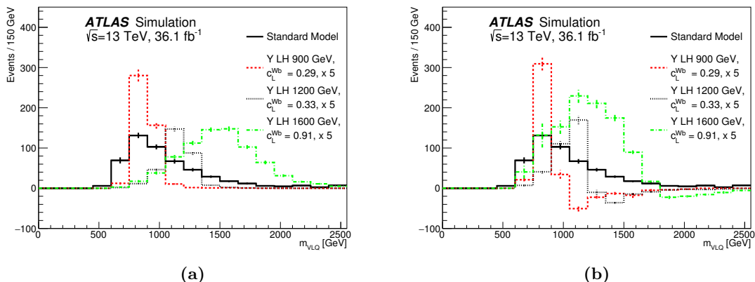
Figure 4. Distribution of VLQ candidate mass, m_{\text{VLQ}} , in the SR for three different signal masses (a) without and (b) with interference effects, for a left-handed Y signal with a mass of 900 GeV (dashed line), 1200 GeV (dotted) and 1600 GeV (dash-dotted line) and a coupling of c_L^{Wb} \approx 0.29 , \approx 0.33 and \approx 0.91 respectively, together with the total SM background (solid line). The error bars represent the statistical uncertainties. The signal event yield is scaled by a factor of five. Depending on the coupling and signal mass it is possible that negative entries occur in some bins of the signal-plus-interference m_{\text{VLQ}} distribution due to the interference effect. The distributions for a right-handed and left-handed Y signal without considering any interference effects are the same.
