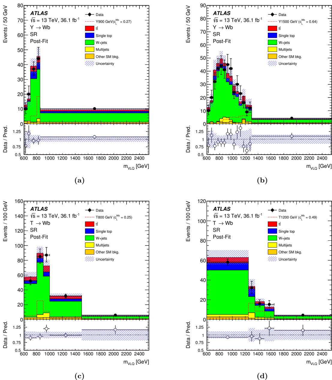
Figure 7. Distributions of the VLQ candidate mass, m_{VLQ} , after the fit to the background-only hypotheses for four different binnings chosen for four different signal masses. The first and last bin include the underflow and overflow respectively. The VLQ candidate mass distributions for (a) a left-handed Y signal with mass 900 GeV and coupling c_L^{Wb} = 0.27 , (b) a left-handed Y signal with mass 1500 GeV and coupling c_L^{Wb} = 0.64 , (c) a left-handed T signal with mass of 800 GeV and coupling c_L^{Wb} = 0.25 and (d) a left-handed T signal with mass 1200 GeV and coupling c_L^{Wb} = 0.49 are also shown; all signal distributions include interference. The lower panels show the ratio of data to the fitted background yields. The error bars represent the statistical uncertainty in the data. The band represents the total systematic uncertainty after the maximum-likelihood fit.
