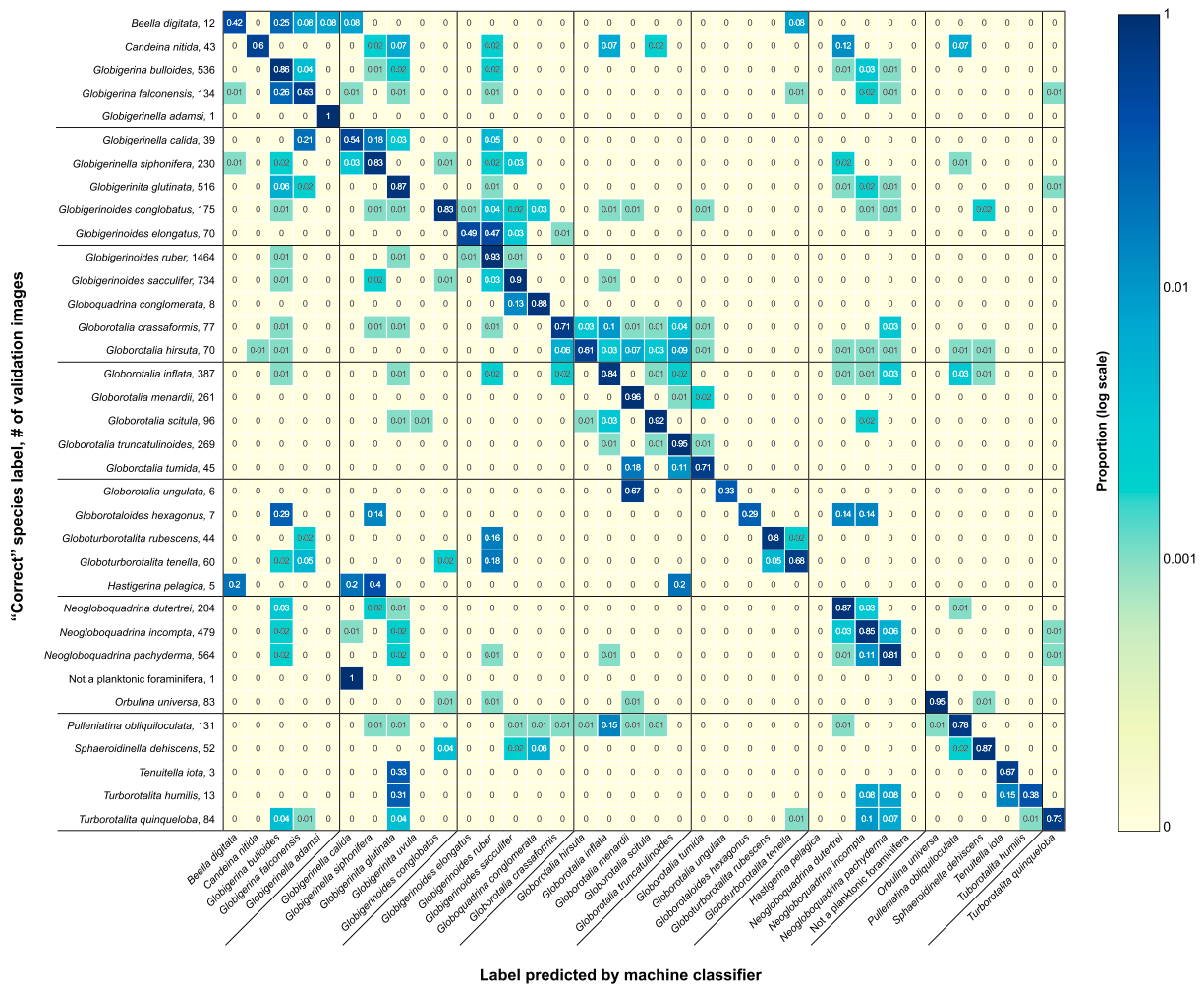
Figure 4. The machine confusion matrix, showing results from the validation set, which contains 80% of the images with high-quality labels from the combined YPM coretop data set and the Buckley data set. The y axis shows the “correct” species labels followed by the number of representative images in the validation set. The x axis shows the corresponding predicted labels, with each matrix cell showing the proportion of validation objects identified as each species (e.g., 86% of the 536 validation images of G. bulloides were correctly identified as G. bulloides and 4% were incorrectly identified as G. falconensis ). The color map is on a log-scale and shows higher (bluer/darker) vs. lower proportions (yellow/lighter).
