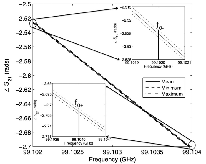
Fig. 18. Impact of uncertainty in \angle S_{21} on the determination on \left| \frac{\partial \angle S_{21}}{\partial \omega} \right| from f_{0+} and f_0 for the strongly-coupled inline PC resonator.
