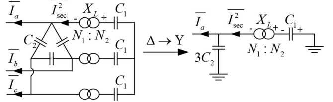
(b) Contribution from the valve side current injection
