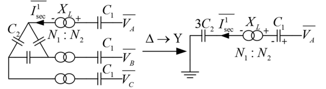
(a) Contribution from the inverter AC bus voltage
