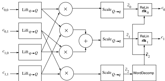
Fig. 2. FV homomorphic multiplication.
