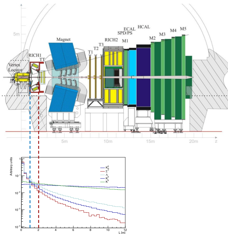
Figure 2. A side view of the LHCb detector layout [16] compared with the decay length of strange hadrons in pp collisions at \sqrt{s} = 13 TeV. The blue (1m) and red (2m) dashed lines indicate the approximate distance from the interaction point at which daughter tracks can be reconstructed as long and downstream tracks, respectively.
