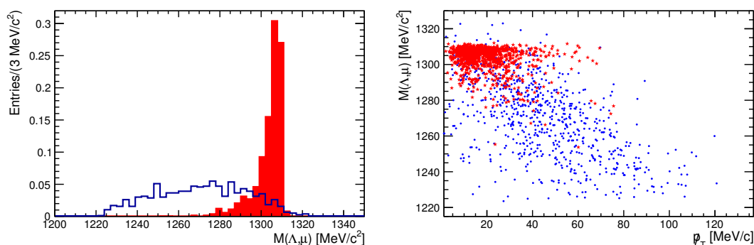
Figure 10. The left plot shows the reconstructed invariant mass for \Xi^- \rightarrow \Lambda\mu^- \bar{\nu}_\mu candidates. Signal events are given by a solid blue line, while the \Xi^- \rightarrow \Lambda\pi^- background is displayed in filled red. The right figure shows a scatter plot of the reconstructed mass vs. missing momentum in the plane transverse to the \Xi^- flight direction for signal (blue squares) and \Lambda \rightarrow p\pi^- background (red stars). Final state radiation in the \Xi^- and \Lambda decay vertices is not included in the simulation.
