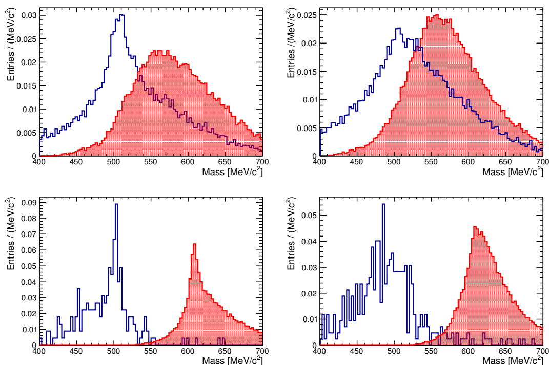
Figure 6. Reconstructed invariant mass for K_s^0 \rightarrow \gamma\mu^+\mu^- (top) and K_s^0 \rightarrow \pi^0\mu^+\mu^- (bottom) obtained from simulation. The K_s^0 \rightarrow \gamma\mu^+\mu^- and K_s^0 \rightarrow \pi^0\mu^+\mu^- signal events are shown with a solid blue line and the K_s^0 \rightarrow \pi^+\pi^- background is illustrated with red filled histograms. The left side portrays events reconstructed with long tracks, while reconstruction with downstream tracks are depicted on the right.
