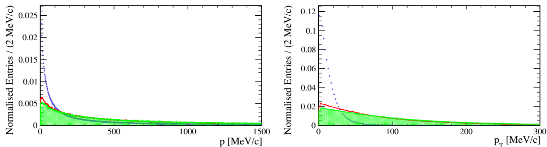
Figure 8. Momentum (left) and transverse momentum (right) for electrons generated in various strangeness decays, where the dotted blue represents \Lambda \rightarrow p\pi^-e^+e^- , solid red K_s^0 \rightarrow \pi^+\pi^-e^+e^- and filled green K_s^0 \rightarrow \mu^+\mu^-e^+e^- .
