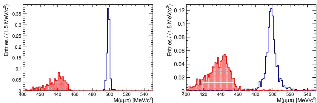
Figure 7. Reconstructed invariant mass for K^+ \rightarrow \pi^+ \mu^+ \mu^- , where signal events are shown with a solid blue line and K^+ \rightarrow \pi^+ \pi^+ \pi^- background illustrated by red filled histograms. The left side gives events reconstructed with long tracks, while reconstruction with downstream tracks are pictured on the right.
