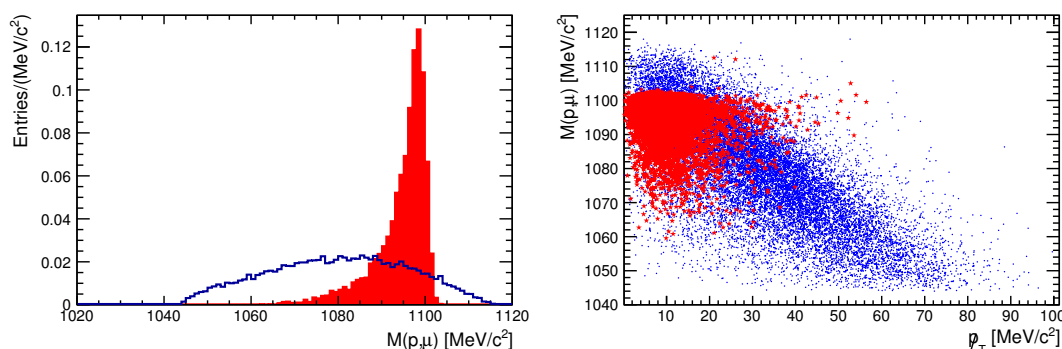
Figure 9. The left plot shows the reconstructed invariant mass for \Lambda \rightarrow p\mu^- \bar{\nu}_\mu candidates. Signal events are given by a solid blue line, while the \Lambda \rightarrow p\pi^- background is displayed in filled red. The right figure shows a scatter plot of the reconstructed mass vs. missing momentum in the plane transverse to the \Lambda flight direction for signal (blue squares) and \Lambda \rightarrow p\pi^- background (red stars). Final state radiation in the \Lambda decay vertex is not included in the simulation.
