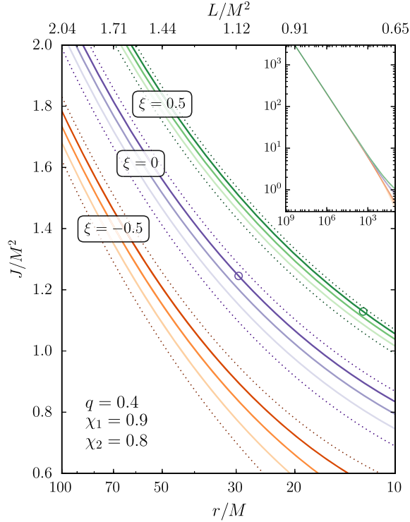
FIG. 7 (color online). Evolution of the total angular momentum magnitude J during the inspiral. Three binary configurations are considered here: \xi = -0.5 (orange), 0 (purple) and 0.5 (green) for q = 0.4 , \chi_1 = 0.9 , \chi_2 = 0.8 . Equation (38) is solved for several different initial conditions (solid lines, sequential colors) as the separation r and the angular momentum L = \eta(rM^3)^{1/2} decrease. Solutions are bounded at all separations by the spin-orbit resonances (dotted lines) which extremize the allowed value of J for fixed \xi . Two of the binaries pictured here cross one of the resonant conditions \alpha = 2\pi n (empty circles) where changes in the direction \hat{\mathbf{J}} are expected. The inset shows the same evolutions for a wider separation range.
