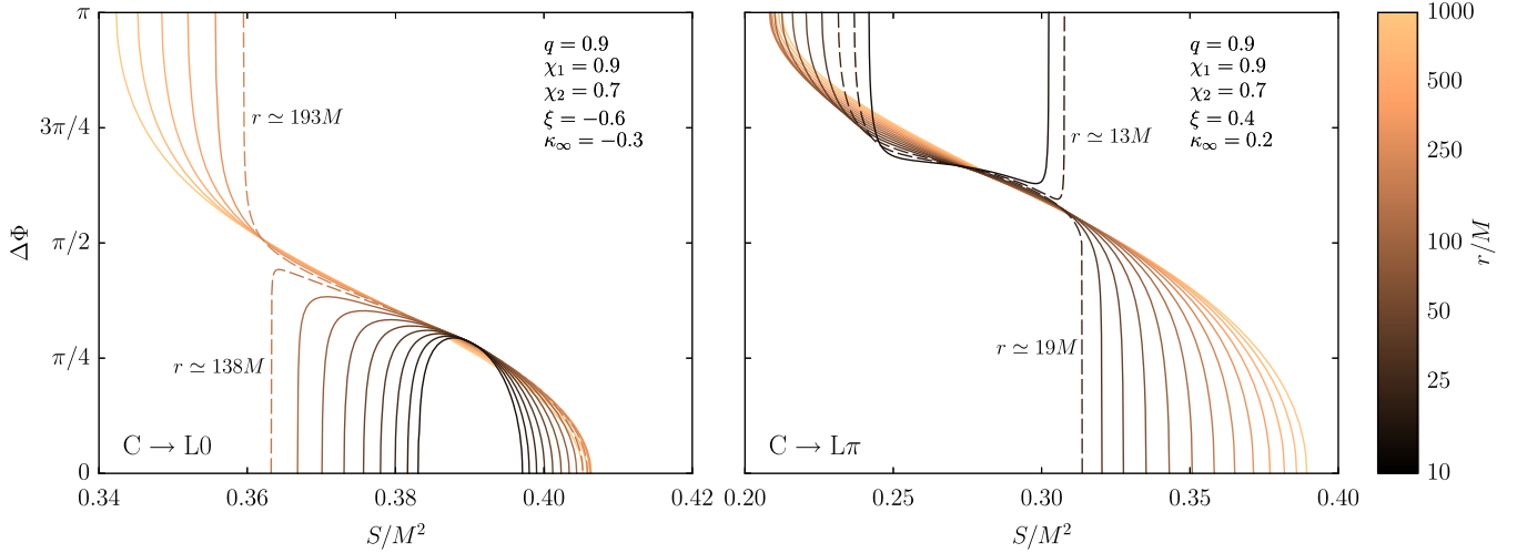
FIG. 10 (color online). Precessional solutions \Delta\Phi(S) of Eqs. (20a)–(20d) as J and L evolve during inspirals according to Eq. (38). These solutions are colored according to the separation r/M as shown in the color bar on the right (orange/lighter for large separations and black/darker for small separations). Binaries in the left (right) panel transition from the circulating morphology to the morphology in which \Delta\Phi librates about 0 ( \pi ) at the transition radius r_{\text{tr}} \approx 152M ( 18.9M ); separations bracketing the transition radius are marked with dashed lines. Parameters are set to the values indicated in the legends. An animated version of this figure is available online [55].
