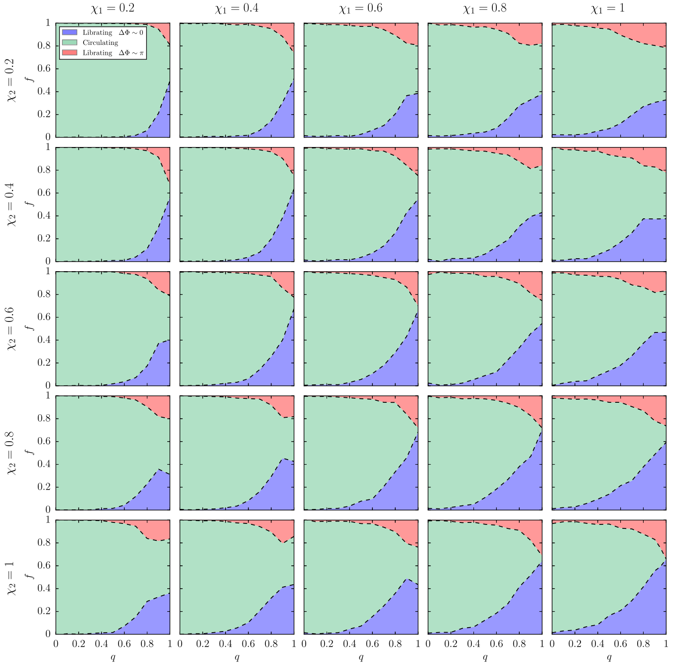
FIG. 13 (color online). The fraction f of isotropic BBHs for which \Delta\Phi circulates (green, middle region), oscillates about 0 (blue, bottom region), or oscillates about \pi (red, top region) at a binary separation r = 10M as functions of the mass ratio q . Dashed lines separate the different morphologies. Each panel corresponds to a different value of \chi_1 (columns) and \chi_2 (rows). The fraction of BBHs in librating morphologies increases as the mass asymmetry decreases ( q \rightarrow 1 ). For nearly equal masses ( q \gtrsim 0.9 ), asymmetry in the spin magnitudes increases the fraction of binaries in the circulating morphology as can be seen by comparing panels on and off the diagonal. Some data used in this plot are listed in Table I. The website [55] contains an animated version of this figure, where the panels are shown at decreasing binary separations.
