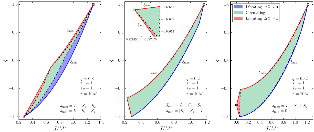
FIG. 5 (color online). The (J, \xi) parameter space for BBHs with different minimum allowed total angular momentum J_{\min} . BBH spin morphology is shown with different colors, as indicated in the legend. The extrema \xi_{\min}(J) and \xi_{\max}(J) of the effective potentials constitute the edges of the allowed regions and are marked by solid blue (red) curves for \Delta\Phi = 0(\pi) . Dashed lines mark the boundaries between the different morphologies. The parameters q, \chi_1, \chi_2 and r are chosen as in Fig. 4, whose panels can be thought of as vertical (constant J ) “sections” of this figure (where we suppress the S dependence). The lowest allowed value of \xi occurs at J = |L - S_1 - S_2| in all three panels. Three phases are present for each vertical section with J > |L - S_1 - S_2| . This condition may either cover the entire parameter space (left panel) or leave room for additional regions where vertical sections include two different phases in which \Delta\Phi oscillates about \pi and a circulating phase in between (center panel) or only a single phase where the spins librate about \Delta\Phi = \pi (right panel). An animated version of this figure evolving on the radiation-reaction time t_{\text{RR}} is available online [55].
