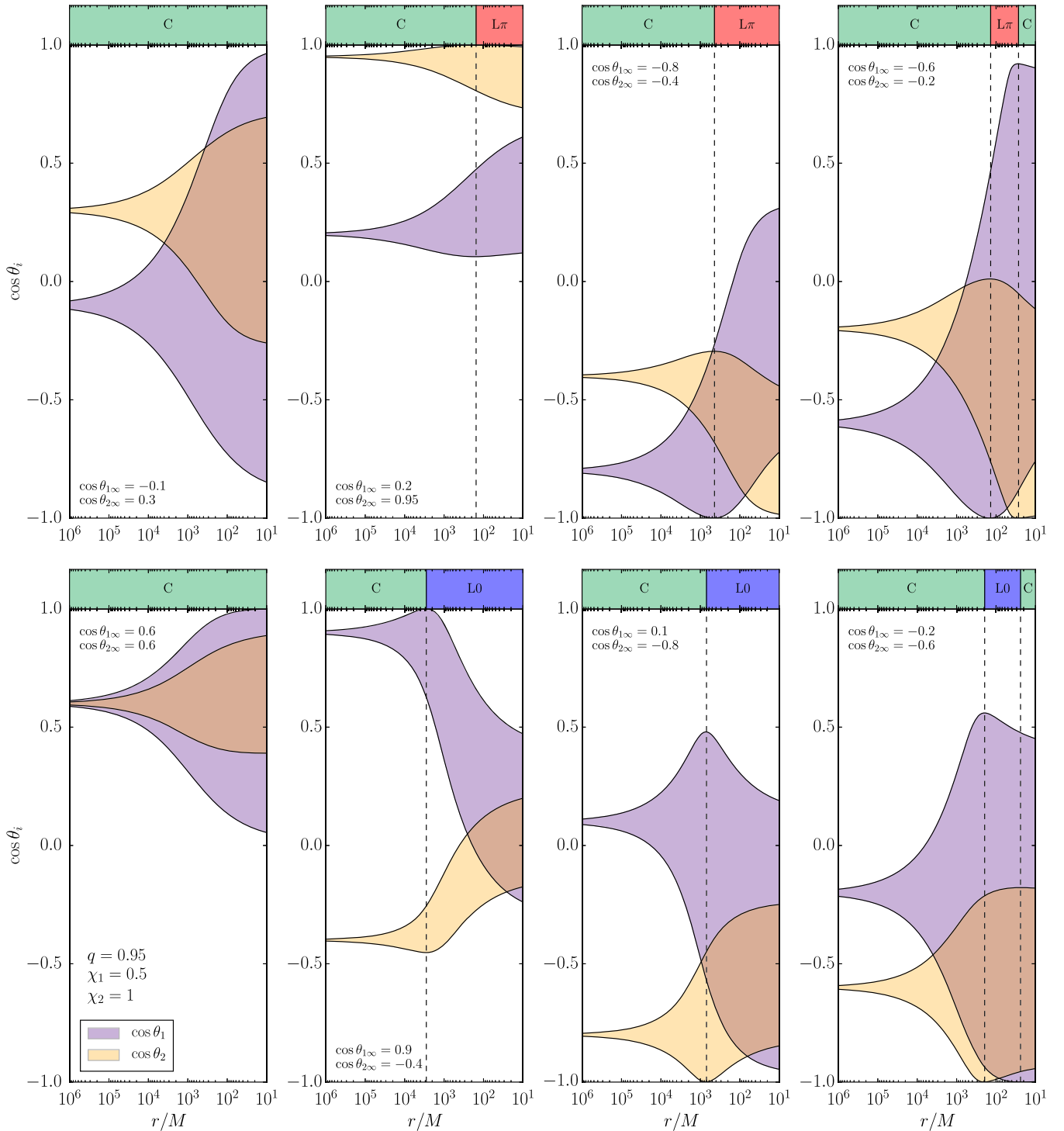
FIG. 11 (color online). Evolution of the spin morphology and the allowed ranges of the spin angles \theta_i over a precession cycle as functions of the binary separation r . Each panel shows the range of \cos \theta_1 (purple/darker) and \cos \theta_2 (orange/lighter) for different initial conditions \cos \theta_{i\infty} . The current morphology is tracked by the horizontal bar above each panel. Morphologies are indicated as C (green) for circulating, L0 (blue) for \Delta\Phi librating about 0, and L \pi (red) for \Delta\Phi librating about \pi . The morphology changes whenever \cos \theta_i = \pm 1 (vertical dashed lines). BBHs in the leftmost column do not undergo any transitions in the PN regime; one transition into a librating morphology occurs for BBHs in the center columns; two transitions (circulating to librating, librating to circulating) occur for BBHs in the rightmost column. The mass ratio and spin magnitudes are q = 0.95 , \chi_1 = 0.5 , and \chi_2 = 1 in all panels.
