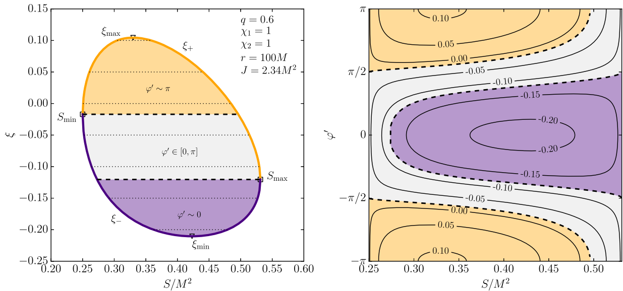
FIG. 2 (color online). Left: Effective potentials \xi_{\pm}(S) for BBHs with q = 0.6 , \chi_1 = \chi_2 = 1 , r = 100M , and J = 2.34M^2 . Conservation of the projected effective spin \xi constrains the BBH spins to precess along horizontal lines bounded by the effective-potential curves. The horizontal dashed lines intersecting the effective potentials at S_{\min} and S_{\max} (marked by empty squares) divide BBH spin precession into three different morphological phases distinguished by whether the angle \varphi' defined by Eq. (9) oscillates about \pi (top orange region), circulates from 0 to 2\pi (middle grey region), or oscillates about 0 (bottom purple region). The effective potentials admit two extrema \xi_{\min} and \xi_{\max} (marked by empty triangles) corresponding to the spin-orbit resonances discovered in Ref. [37]. Right: Contours of constant \xi(S, \varphi') given by Eq. (13) for the same binary parameters. As BBH spins precess along the horizontal dashed lines in the left panel, they move along the curves in the S\varphi' plane in the right panel illustrating the three morphological phases.
