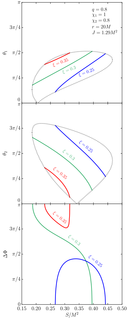
FIG. 3 (color online). Analytical solutions given by Eq. (20) for the evolution of the angles \theta_1 (top panel), \theta_2 (middle panel), and \Delta\Phi (bottom panel) during a precession cycle. The evolution of three binaries with \xi = 0.25 (blue), 0.3 (green) and 0.35 (red) is shown for q = 0.8 , \chi_1 = 1 , \chi_2 = 0.8 , r = 20M and J = 1.29M^2 . The evolution of \theta_1 and \theta_2 is monotonic during each half of a precession cycle and is bounded by the dotted lines for which \cos\varphi = \mp 1 [these curves can be found by substituting \xi_{\pm}(S) for \xi in Eq. (20)]. Three classes of solutions are possible and define the binary morphology: \Delta\Phi can oscillate about 0 ( \xi = 0.25 ), circulate ( \xi = 0.3 ) or oscillate about \pi ( \xi = 0.35 ). An animated version of this figure is available online at Ref. [55], where precession solutions are evolved on t_{RR} .
