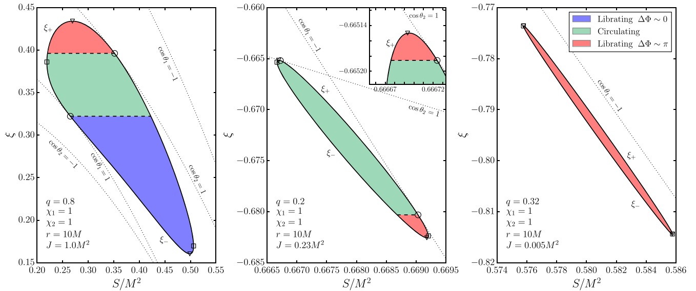
FIG. 4 (color online). Effective potentials \xi_{\pm}(S) of Eq. (14) for values of L , J , S_1 , and S_2 leading to three different sets of spin morphologies. The loop formed by the two curves encloses all allowed configurations for the constants listed in the legends. As in the left panel of Fig. 2, empty squares mark the extrema of S ( S_{\min} and S_{\max} ), empty triangles mark the extrema of \xi ( \xi_{\min} and \xi_{\max} ), and conservation of \xi restricts the BBH spins to precess along horizontal lines between the turning points S_{\pm} . BBH spin precession can be classified into three different morphologies by the behavior of \Delta\Phi during a precession cycle: oscillation about 0 (blue region), circulation from -\pi to \pi (green region), or oscillation about \pi (red region). The dashed boundaries between these morphologies occur at values of \xi where the dotted curves \cos\theta_i = \pm 1 intersect the effective-potential loop, as shown by the empty circles. All three morphologies are present if one intersection occurs on \xi_+(S) and a second occurs on \xi_-(S) (left panel), oscillation of \Delta\Phi about 0 is forbidden if two intersections occur on either \xi_+(S) or \xi_-(S) (middle panel), and only oscillations about \pi are allowed if there are no such intersections (right panel).
