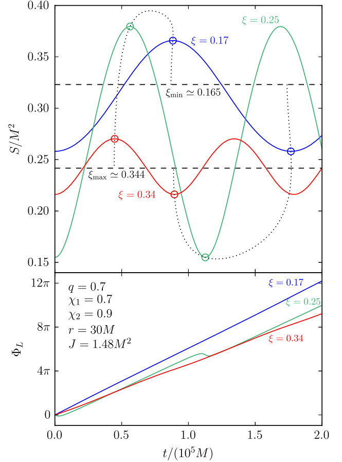
FIG. 6 (color online). Time-dependent solutions for the total spin magnitude S (top panel) and the orbital-angular-momentum phase \Phi_L (bottom panel). We set q = 0.7 , \chi_1 = 0.7 , \chi_2 = 0.9 , r = 30M and J = 1.48M^2 and integrate Eq. (26) for three values of \xi corresponding to the three different spin morphologies: \Delta\Phi oscillates about 0 ( \xi = 0.17 , blue), circulates ( \xi = 0.25 , green), and oscillates about \pi ( \xi = 0.34 , red). Initial conditions have been chosen such that S = S_- and \Phi_L = 0 at t = 0 . The oscillations in S induce small wiggles in \Phi_L on top of a mostly linear drift. Spin-orbit resonances (horizontal dashed lines, top panel) correspond to configurations for which S is constant and can be interpreted as zero-amplitude limits of generic oscillatory solutions. The projections of the effective potentials, i.e. parametric curves [\tau(\xi)/2, S_+(\xi)] and [\tau(\xi), S_-(\xi)] , are shown with dotted lines. An animated version of this figure is available online [55].
