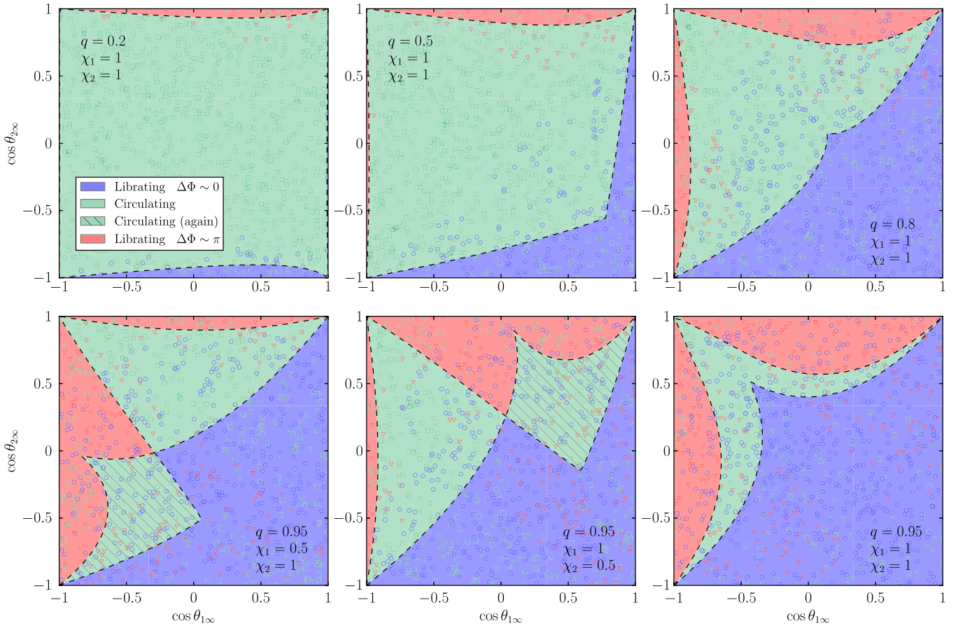
FIG. 14 (color online). Spin morphologies at r_f = 10M as functions of the asymptotic values of the spin angles \theta_{i\infty} . The mass ratio q and spin magnitudes \chi_i for each panel are indicated in the legends. Evolving BBHs along the four lines \cos\theta_i = \pm 1 at r_f out to r/M \rightarrow \infty using our new precession-averaged approach yields the dashed curves separating the different final morphologies: \Delta\Phi oscillates about 0 (blue), oscillates about \pi (red), circulates without ever having experienced a phase transition (plain green), or circulates after having experienced a phase transition to libration and then a second phase transition back to circulation (hatched green). The morphology within each region defined by the dashed boundaries is determined by which of the conditions \cos\theta_i = \pm 1 these boundaries satisfy, as described in Sec. IV C. The points show the locations of binaries in the \cos\theta_1 - \cos\theta_2 plane at r_f and are colored by their morphology at that separation [ \Delta\Phi oscillates about 0 (blue circles), oscillates about \pi (green squares), or circulates (red triangles)]. Because morphology depends on \Delta\Phi in addition to \theta_1 and \theta_2 at finite separation, the projection onto the \cos\theta_1 - \cos\theta_2 plane can lead points of different morphologies to occur at the same positions, particularly for comparable-mass binaries q \approx 1 where the \theta_i 's oscillate with greater amplitude. The website [55] contains an animated version of this figure in which r_f evolves.
