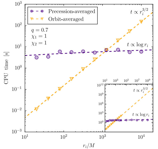
FIG. 9 (color online). CPU time needed to evolve BBHs from an initial separation r_i to a final separation r_f = 10M using our new precession-averaged approach (purple circles) and the standard orbit-averaged approach (orange triangles). Each CPU time is averaged over N = 100 executions with isotropic initial spin orientation (flat distributions in \cos\theta_1 , \cos\theta_2 and \Delta\Phi ). Dashed lines show the expected scalings: t \propto r_i^{3/2} for the orbit-averaged approach and t \propto \log r_i for our new precession-averaged approach. These computations have been performed on a single core of a 2013 Intel i5-3470 3.20 GHz CPU.
