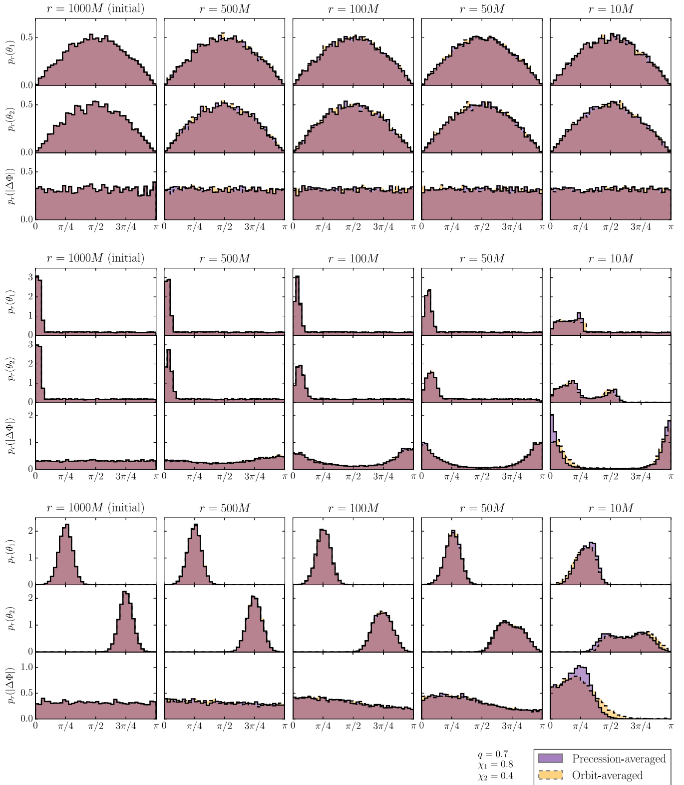
FIG. 8 (color online). Precession-averaged BBH inspirals as described in Sec. III C (purple/darker) compared to numerical integration of the orbit-averaged PN equations [35,36] (orange/lighter). Marginalized distributions of the spin angles \theta_1 , \theta_2 , and |\Delta\Phi| (rows) are shown at several separations along the inspirals [columns: r_i = 1000M , 500M , 100M , 50M , and 10M ]. The three initial spin distributions are isotropic (top panels), one aligned BH (middle panels), and Gaussian spikes (bottom panels) as described in Sec. III C. The two approaches are in good agreement except for minor deviations in the distribution of \Delta\Phi at r \sim 10M . We take q = 0.7 , \chi_1 = 0.8 and \chi_2 = 0.4 for all BBHs. An animated version of this figure is available online [55].
