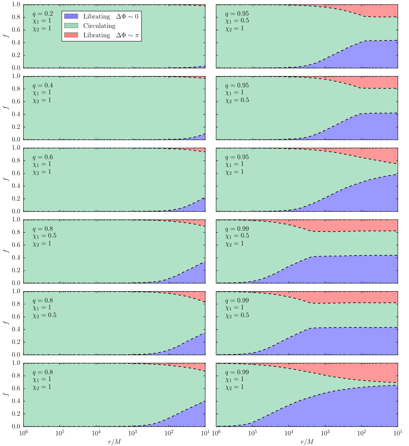
FIG. 12 (color online). The fraction f of isotropic binaries in each of the three precessional morphologies as functions of the binary separation. Each panel refers to different values of q , \chi_1 and \chi_2 as indicated in the legends. The fraction of binaries in which \Delta\Phi circulates (green, middle region of each panel), oscillates about 0 (blue, bottom region of each panel), or oscillates about \pi (red, top region of each panel) is shown as the binary orbit shrinks, with dashed lines separating the different morphologies. The fraction of binaries in librating morphologies generally grows during the inspiral; this growth is stronger as q \rightarrow 1 but may stall for nearly equal masses and \chi_1 \neq \chi_2 , as seen in panels in the right column.
