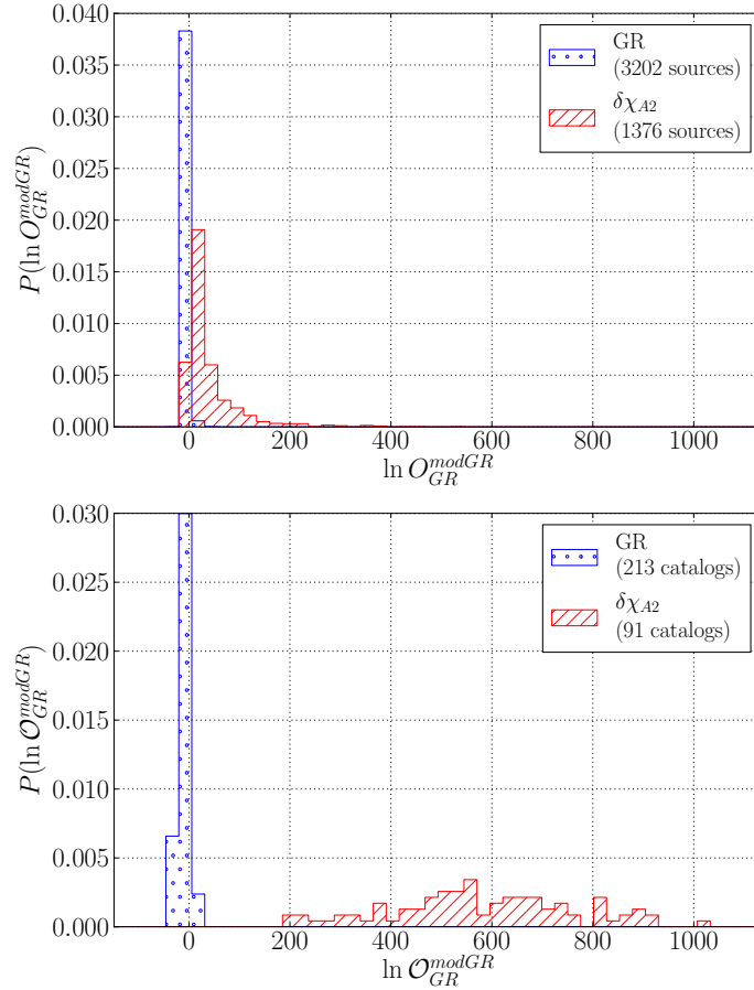
Figure 7.3. Background (blue) and the foreground (red) for a deviation as in Eq. (7.22). The top plot show the results for single sources, whereas the bottom plot shows the results for catalogs of 15 sources.
