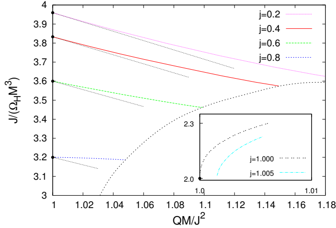
Figure 3.4. The scaled moment of inertia \hat{I} = J/(\Omega_H M^3) is shown versus the scaled quadrupole moment \hat{Q} for fixed values of j . The Kerr BHs are indicated by the fat dots on the \hat{I} -axis. The straight dotted lines represent the perturbative results of [76]. The critical BHs are represented by the dotted curve. [From [82].]
