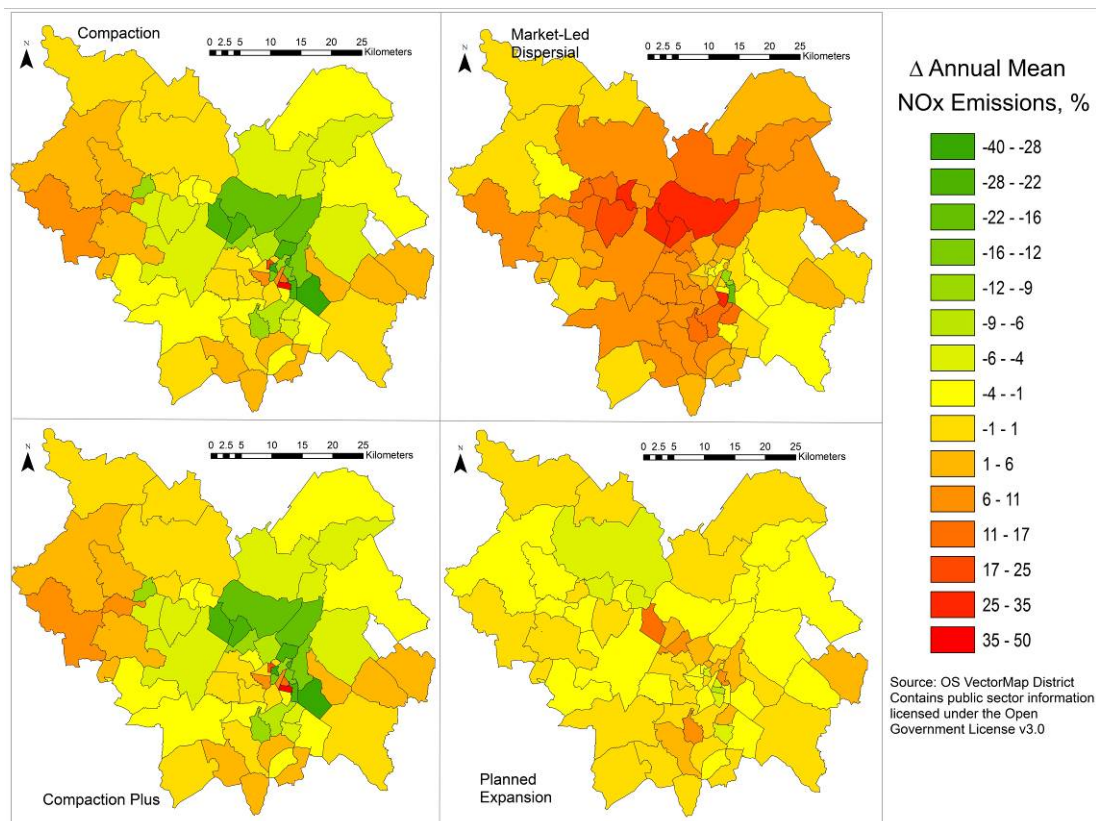
Figure 6: Spatial changes in NO x emissions across Cambridgeshire, relative to the 'Trend' scenario (Anti-clockwise from top left: Compaction, Compaction+, Planned Expansion, Market-led Dispersal)
