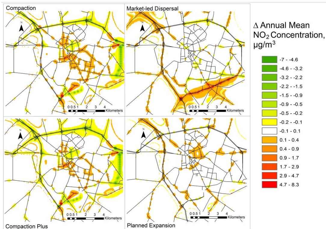
Figure 7: Changes in predicted annual mean \text{NO}_2 concentrations across the City of Cambridge, relative to the 'Trend' scenario (Anti-clockwise from top-left: Compaction, Compaction Plus, Planned Expansion and Market-led Dispersal)
