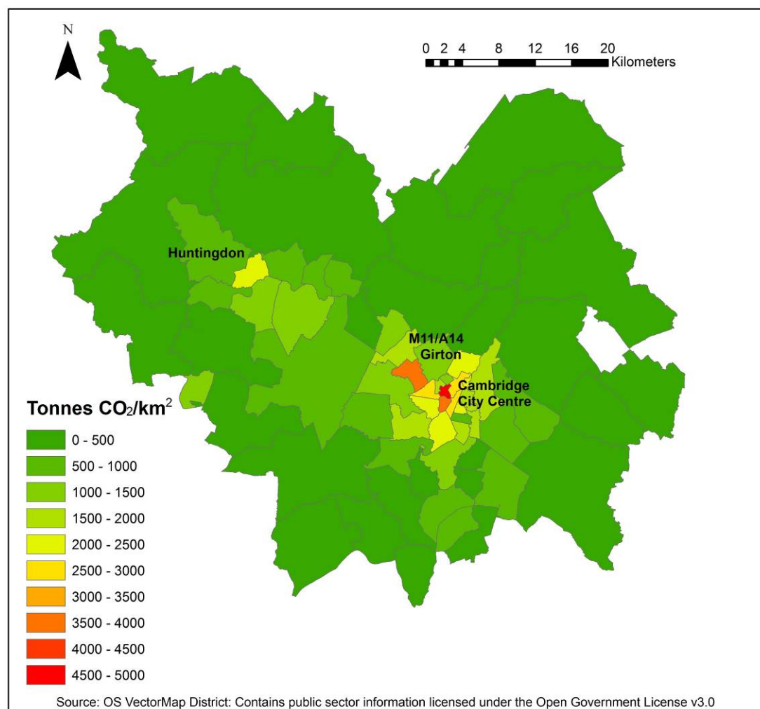
Figure 5: Intensity of CO 2 emissions across the modelled sub-region
