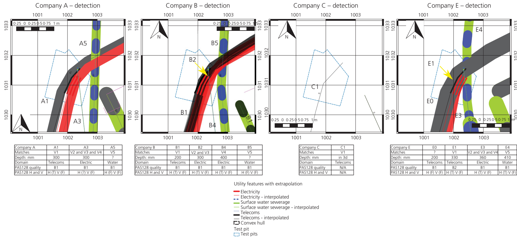
Figure 10. Location of trial pit 10 with the detected features and verified, by excavation for (a) company A, (b) company B, (c) company C and (d) company E
