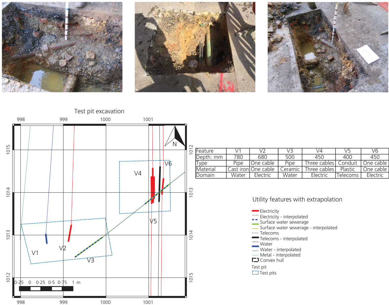
Figure 7. Trial pits 8 and 18 showing the exposed assets together with the verified depth information and the photos taken on the day
