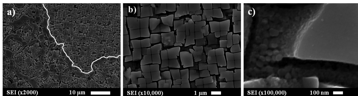
Fig. 4. SEI-SEM micrographs showing the phases present in the as-HIPped CM247LC: (a) Necklace structure of coarse \gamma' at grain boundaries (outlined in white for the large grain at the top right of the image) with fine \gamma' in the grain interior, (b) high magnification image of the fine (1 \mu\text{m} ) \gamma' with irregular cuboidal morphology, and (c) ultra-fine tertiary \gamma' .
