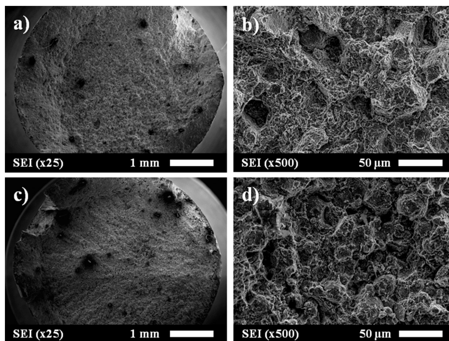
Fig. 14. Fracture surfaces from the ET tensile tests for the sieved powders. The \text{S}_\text{C} powder (a,b) exhibited the best ductility in the current work resulting in (a) fracture surfaces with large shear lips ductile and (b) transgranular fracture. The \text{S}_\text{F} powder (c,d) exhibited (c) much bigger shear lips than the unsieved fine powder, and (d) much more ductile fracture surface showing microvoid coalescence and free from PPBs.
