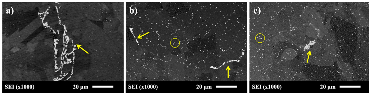
Fig. 5. SEI-SEM micrographs of the Hf+O rich inclusions (arrowed) and (Hf,Ta)-rich fine particles (circled), showing (a) large and irregular particles/clusters sometimes found within the coarse powder, (b) similar, but generally finer clusters in the wide range powder, and (c) localised clusters in the fine powder. The chemical analysis of the different particles is given in Table 4.
