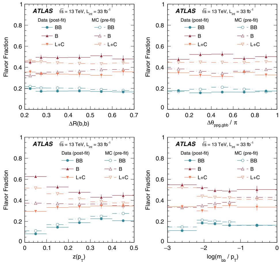
FIG. 5. The prefit (MC) and postfit (data) flavor fractions for \Delta R(b, b) (top left), \Delta\theta_{ppg,gb} (top right), z(p_T) (bottom left), and \log(m_{bb}/p_T) (bottom right) are indicated with open and solid markers respectively. The error bars include only statistical uncertainties from the flavor-fraction fit. The fit's systematic uncertainties are comparable in magnitude, but correlated across the bins. The impact of both the flavor-fraction fit's statistical and systematic uncertainties on the final results is presented in Table I.
