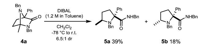
Scheme 2 Reductive ring opening of 4a .
