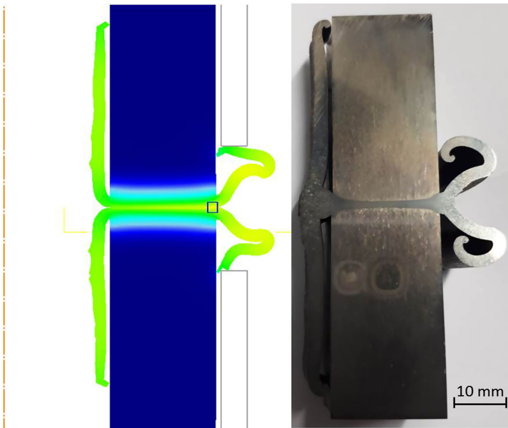
Fig. 5—Comparison of macroscale flash appearances within the model and the real process.
