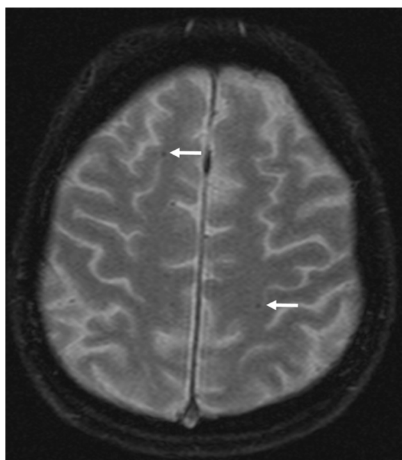
Fig. 2 T2*-weighted imaging depicting multiple cerebral microbleeds (indicated by arrows) in a man aged 71 years with known AF and coronary artery occlusive disease (CHA 2 DS 2 -VASC-score = 2)
