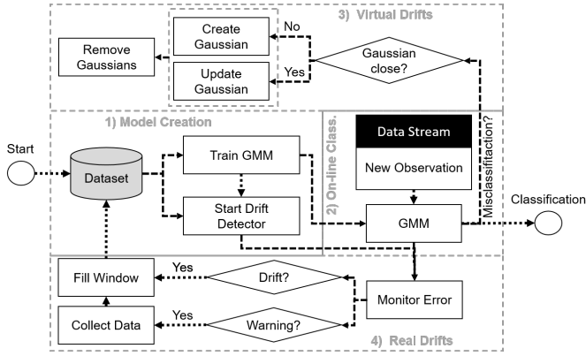
Fig. 1: GMM-VRD's Overall Procedure.
