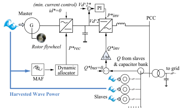
Fig. 3 System control based on a moving average filter (MAF)
