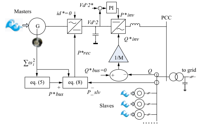
Fig. 6 System control based on the energy filter (EF)
